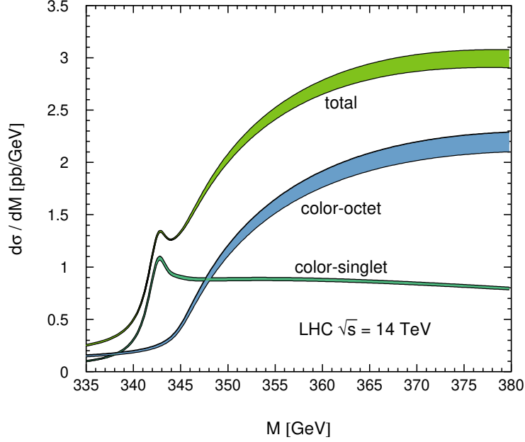
Figure 2.3.: Differential cross-section of top-quark pair production in a colour-singlet or -octet state. The Figure is taken from Reference [37], which provides further details on the underlying modelling.
