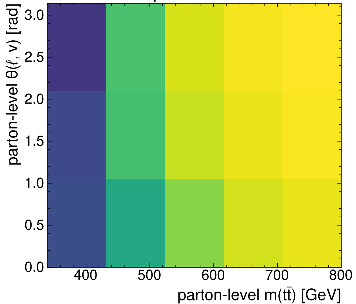
CompactTransformer
