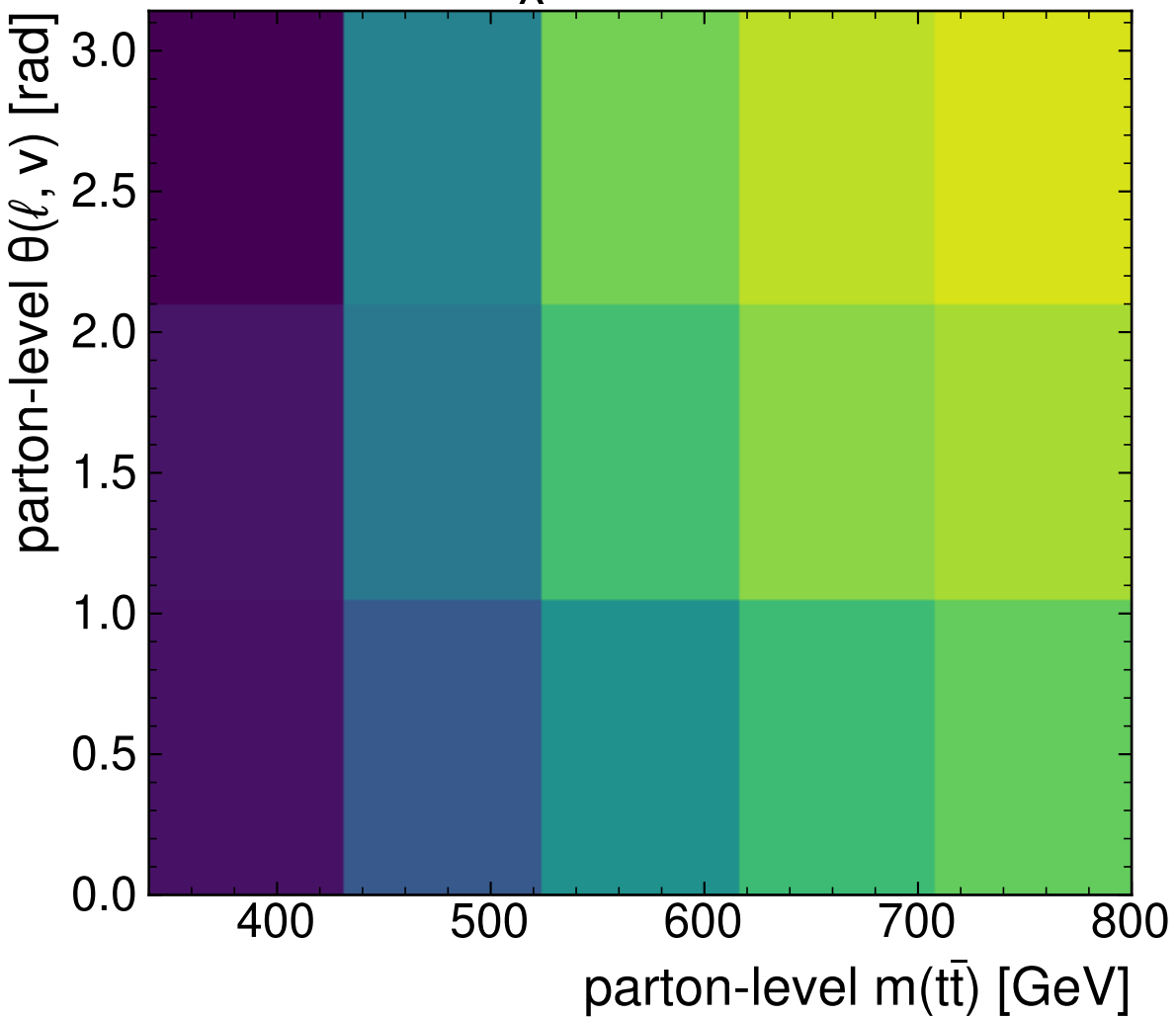
MultiModalTransformer
