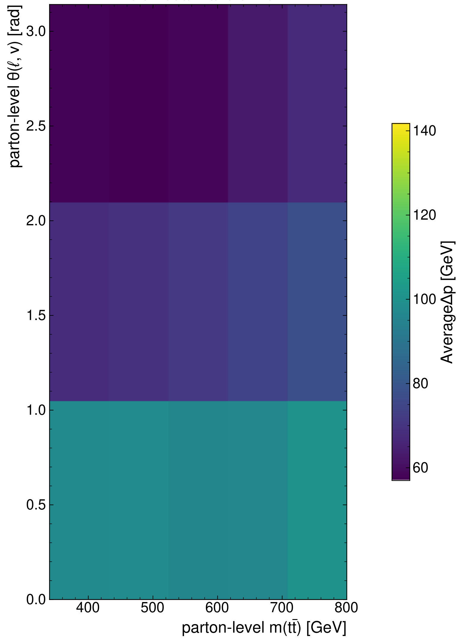
MultiModalTransformer
