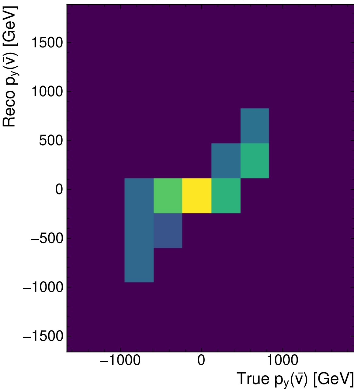
MultiModalTransformer
