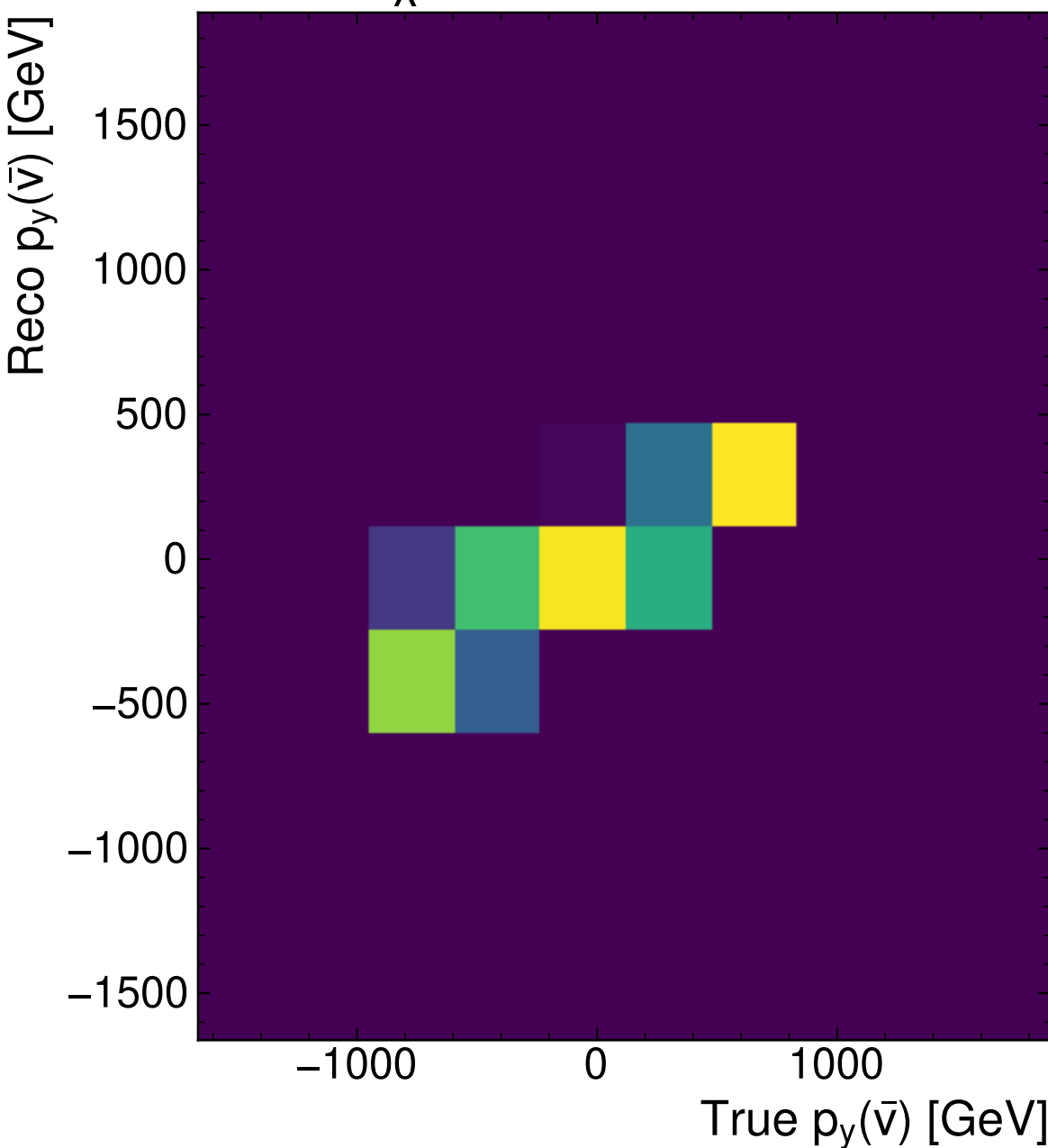
MultiModalTransformer
