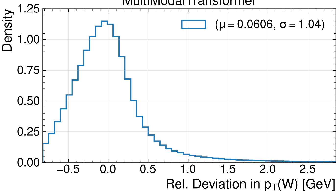
MultiModalTransformer
