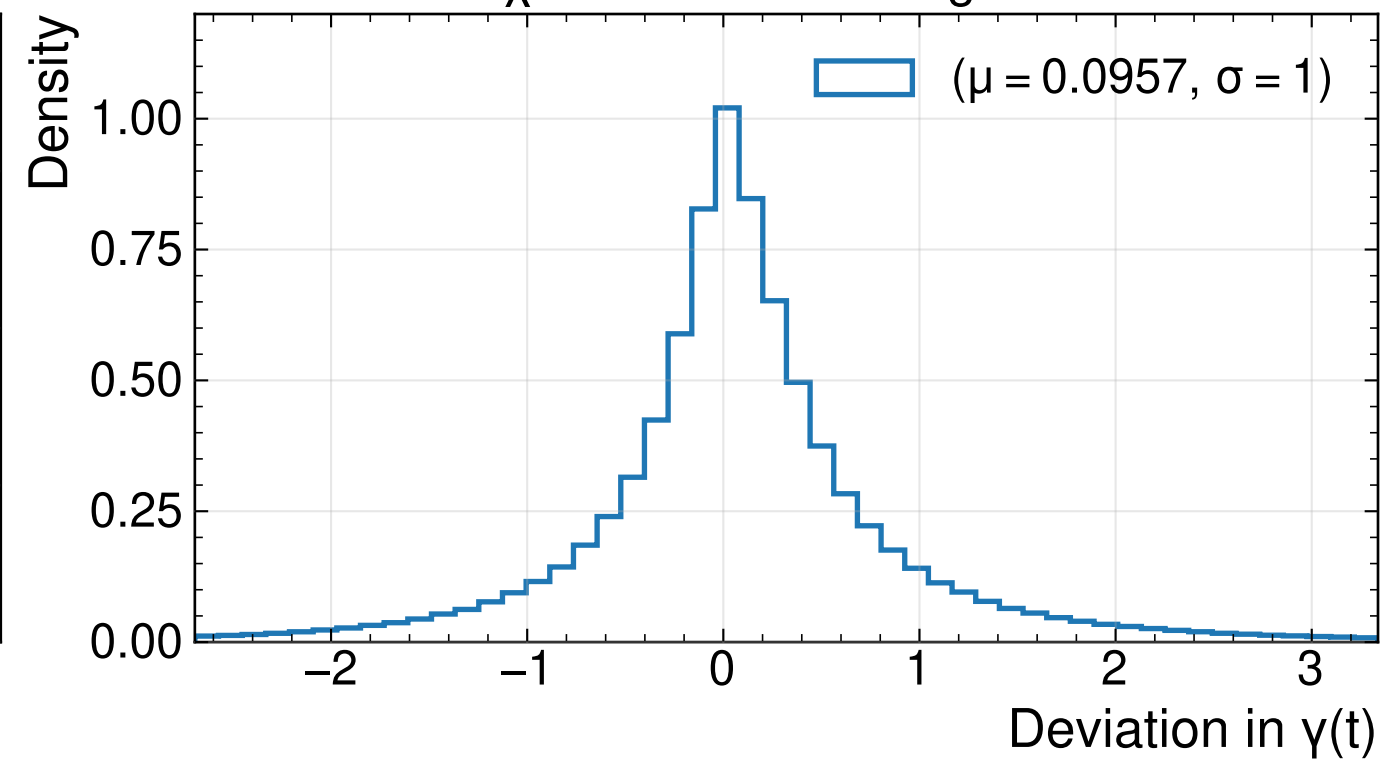
\chi^2 -Method + v-Weighter
