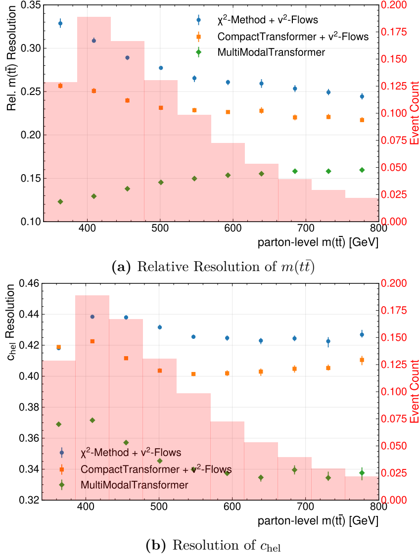
Figure 7.14.: (Relative) Resolution of m(tt) (a) and c_{hel} (b) computed in bins of the parton-level invariant mass of the tt -system. Different setups for assignment and regression are compared.
