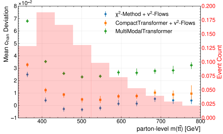
(b) Mean Deviation of c_{\text{chan}}
