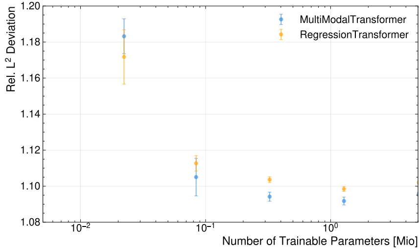
Figure 6.12.: Relative 2-norm deviation of the predicted neutrino momenta compared to RegressionTransformer, which features the same architecture trained only for the neutrino regression task, as a function of the number of trainable parameters.
