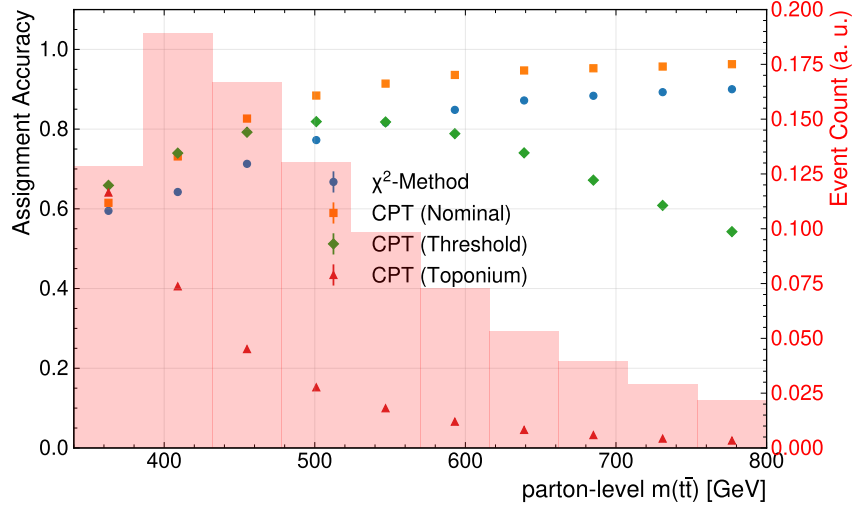
Figure A.25.: Assignment accuracy for different methods computed in bins of the parton-level invariant mass of the t\bar{t} system. The brackets describe the dataset used in the training of the MMT: Nominal with t\bar{t}_{\text{pQCD}} events, Toponium with t\bar{t}_{\text{NRQCD}} events, and Threshold with t\bar{t}_{\text{pQCD}} events with m(t\bar{t}) < 450 GeV. The background histogram shows the distribution of events as a function of the number of jets. The uncertainties represent the statistical variations in the evaluation dataset.
