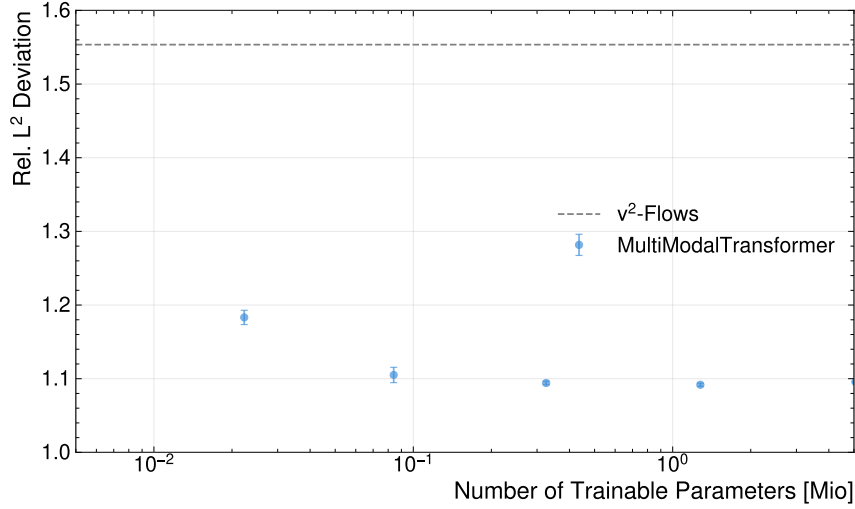
Figure 6.8.: Relative 2-norm deviation of the predicted neutrino momenta compared to the true values as a function of the number of trainable parameters for the MMT architecture with \nu^2 -Flows plotted for comparison.
