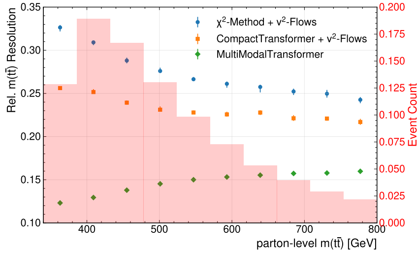
Figure 7.12.: Relative Resolution of m(t\bar{t})
