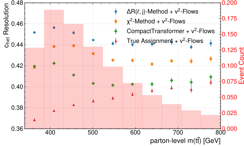
Figure 7.8.: Resolution of c_{\text{hel}}
