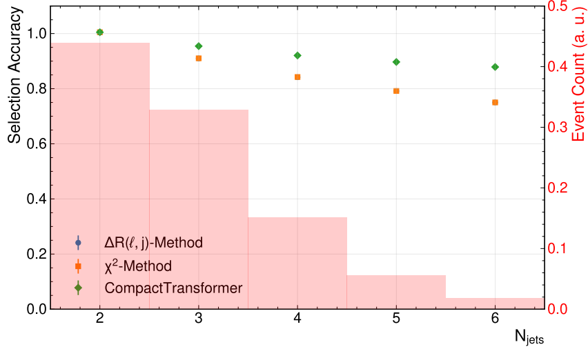
Figure A.14.: Selection accuracy as a function of the number of jets in the event for different reconstruction methods. The background histogram shows the distribution of events as a function of the number of jets. The uncertainties represent the statistical variations in the evaluation dataset.
