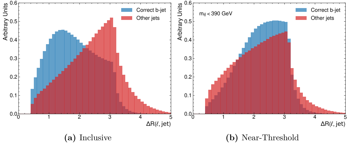
Figure A.3.: Distribution of \Delta R(\ell, j) for correct and incorrect pairing of jets and leptons. Evaluated on the full sample in (a) and near-threshold in (b).
