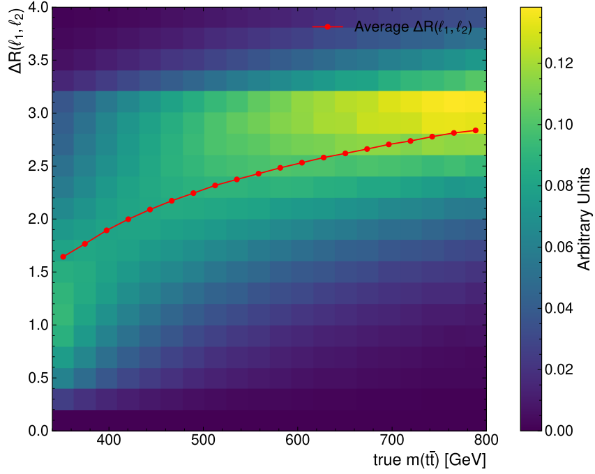
Figure A.2.: This plot shows the distribution of events binned in the parton-level m(t\bar{t}) and the angular distance \Delta R(\ell_1, \ell_2) .
