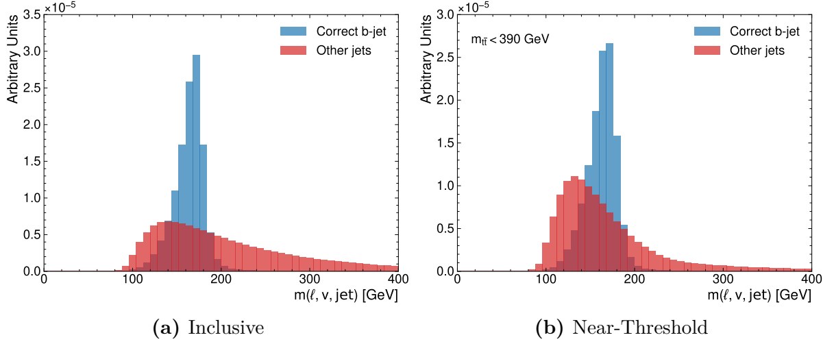
Figure A.4.: Distribution of m(\ell, \nu, j) for correct and incorrect pairing of jets and leptons. Evaluated on the full sample in (a) and near-threshold in (b).
