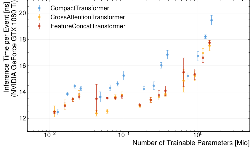
Figure 6.5.: Inference Time of all architectures as a function of the number of trainable parameters. Each point represents the average inference time across 5 runs with different random seeds and k-fold training/validation splits. The error bars indicate the standard deviation across the runs. Note that the x-axis is logarithmic, which allows better visualisation of performance differences across model sizes.
