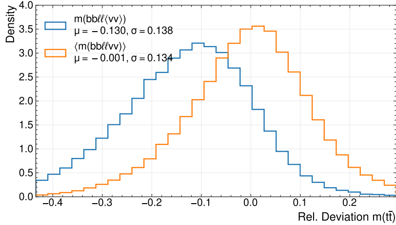
Figure 7.18.: Relative deviation between the reconstructed and true m(t\bar{t}) of the MMT trained with a Gaussian-Loss. The different curves show whether the invariant mass was computed using the mean momentum or by propagating the neutrino probabilities and averaging of obtained masses.
