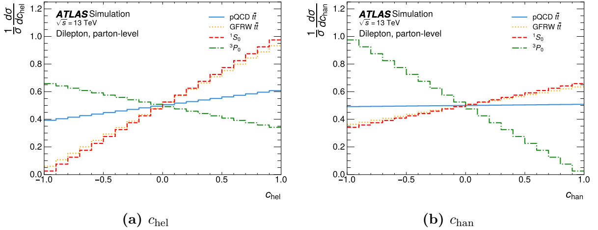
Figure 2.5.: Simulation of the distributions of c_{\text{hel}} and c_{\text{han}} for dileptonic decaying top-quark pairs produced near threshold for different spin states and combinations thereof. The distributions are normalised to unity and computed at parton level. The Figures are taken from Reference [2].
