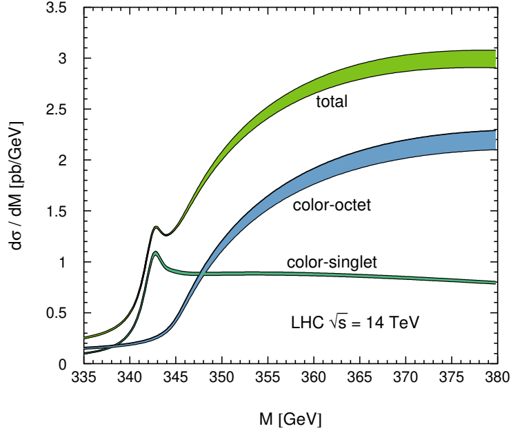
Figure 2.3.: Differential cross-section of top-quark pair production in a colour- singlet or -octet state. The Figure is taken from Reference [37], which provides further details on the underlying modelling.
