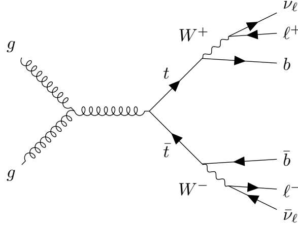
Figure 2.4.: Leading order Feynman diagram for top-quark pair production via gluon fusion with dileptonic decay.
