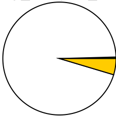
dilep_assigner_sr8
