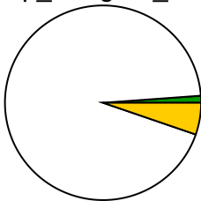
dilep_assigner_sr3
