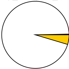
dilep_assigner_sr7
