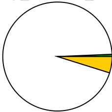
dilep_assigner_sr6
