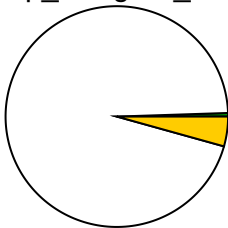
dilep_assigner_sr4
