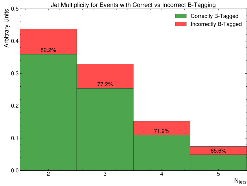
Figure A.1.: This plot shows the b-tagging performance for different numbers of jets in the event. For each jet multiplicity, the number of events, with only jets from top-decays being b-tagged
