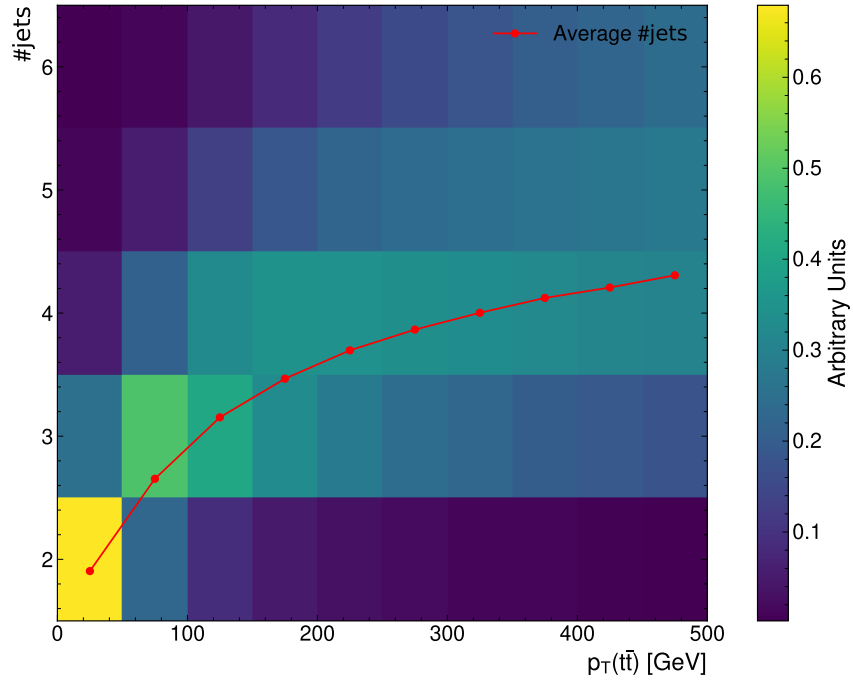
Figure A.3.: This plot shows the distribution of events binned in the parton-level p_T(t\bar{t}) and number of jets per event.
