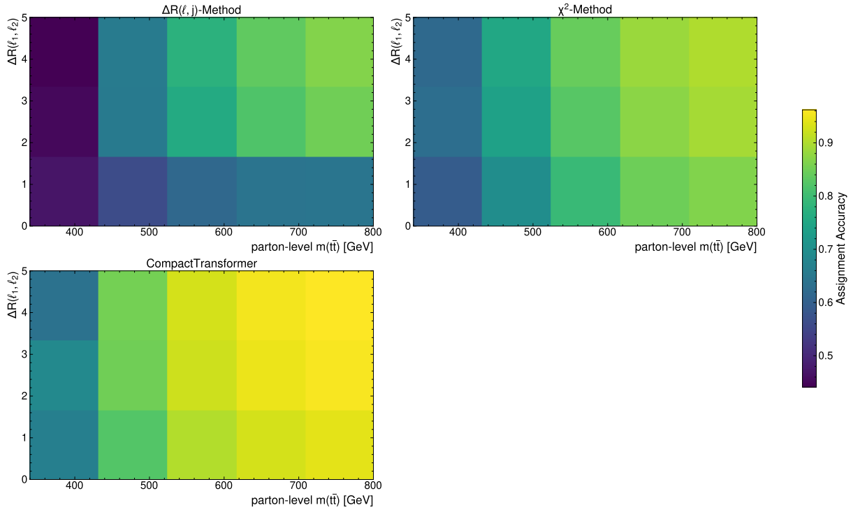
Figure A.11.: Assignment accuracy binned with respect to parton-level m(t\bar{t}) and \Delta R(\ell_1, \ell_2) .
