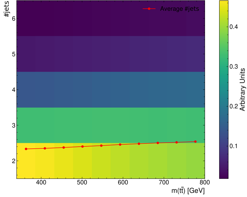
Figure A.2.: This plot shows the distribution of events binned in the parton-level m(t\bar{t}) and number of jets per event.
