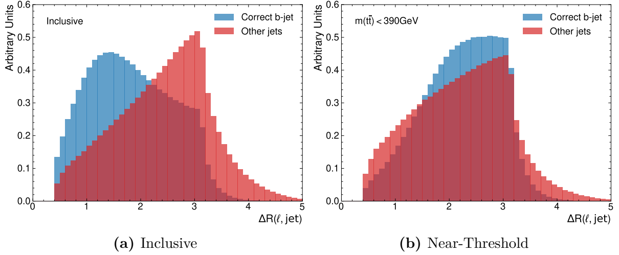
Figure A.5.: Distribution of \Delta R(\ell, j) for correct and incorrect pairing of jets and leptons. Evaluated on the full sample in (a) and near-threshold in (b).
