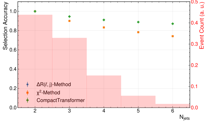
Figure A.10.: Selection accuracy as a function of the number of jets in the event for different reconstruction methods. The background histograms show of the distribution of events as a function of the number of jets. The uncertainties represent the statistical variations in the evaluation dataset.
