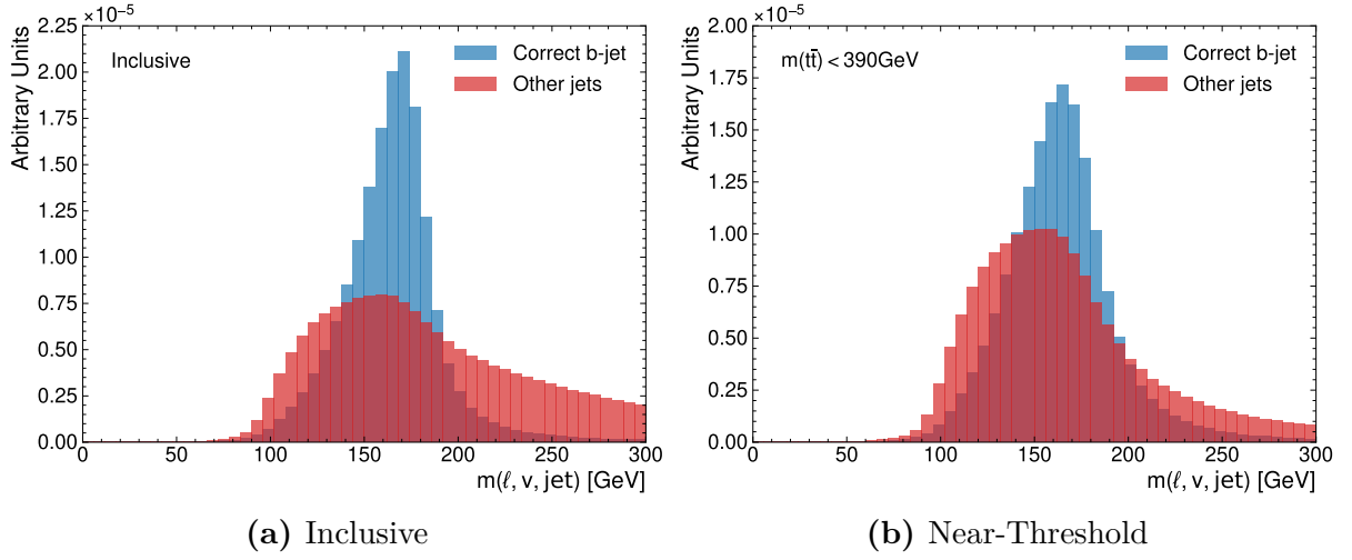
Figure A.6.: Distribution of m(\ell, \nu, j) for correct and incorrect pairing of jets and leptons. Evaluated on the full sample in (a) and near-threshold in (b). Note, that the regressed neutrino momenta from nu^2 -Flows were used.
