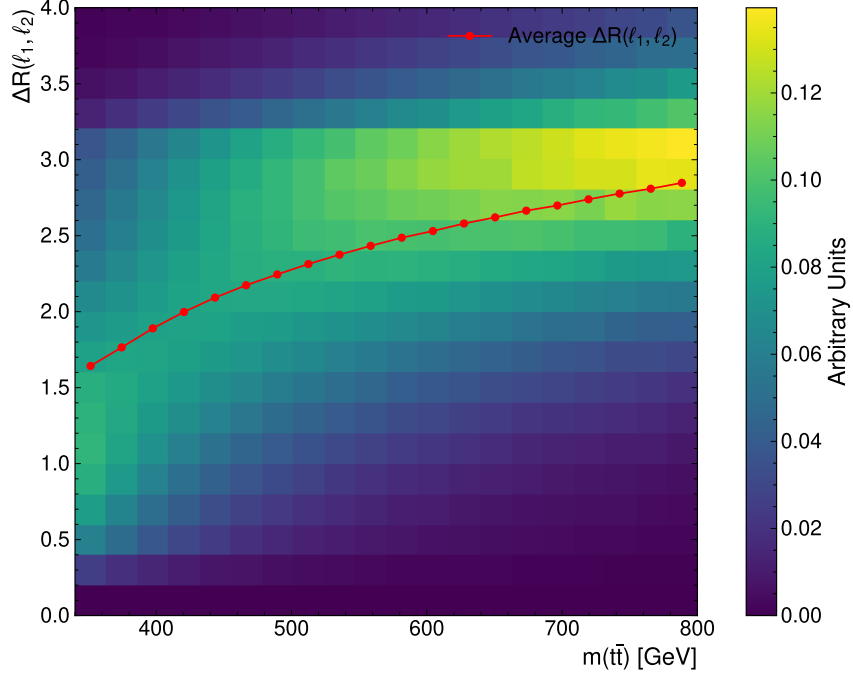
Figure A.4.: This plot shows the distribution of events binned in the parton-level m(t\bar{t}) and the angular distance \Delta R(\ell_1, \ell_2) .
