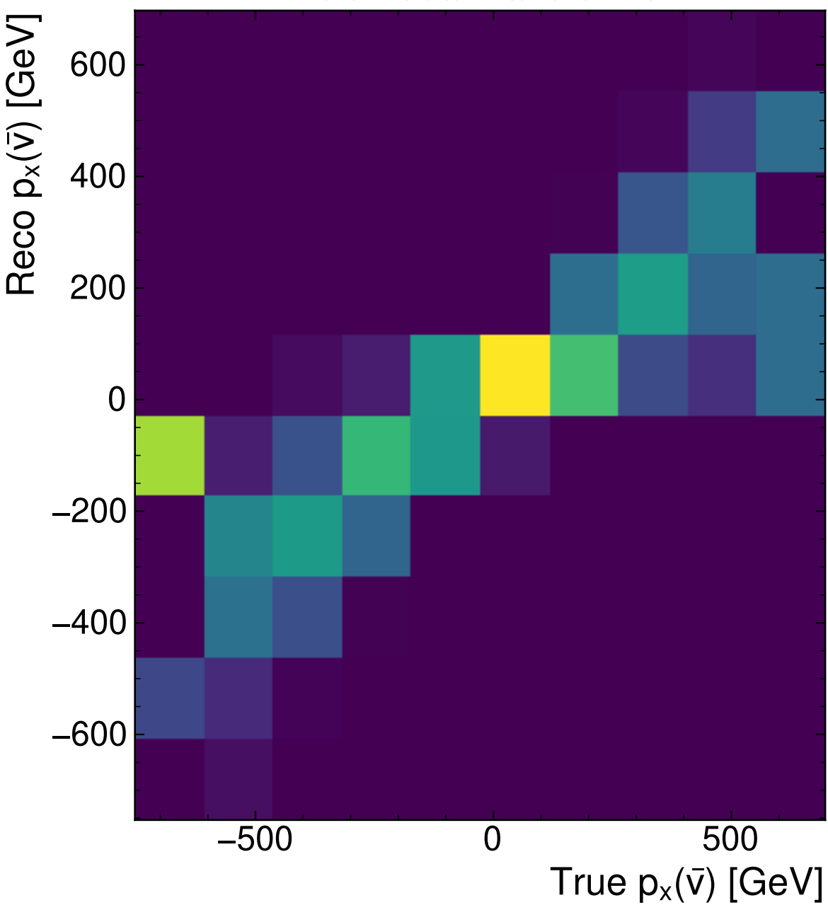
MultiModalTransformer
