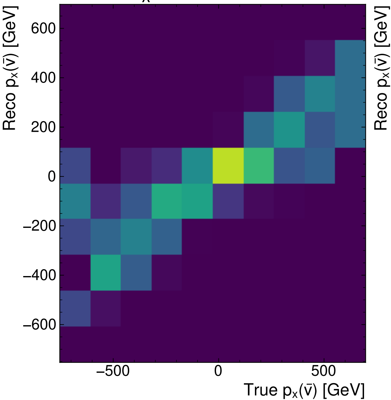
MultiModalTransformer
