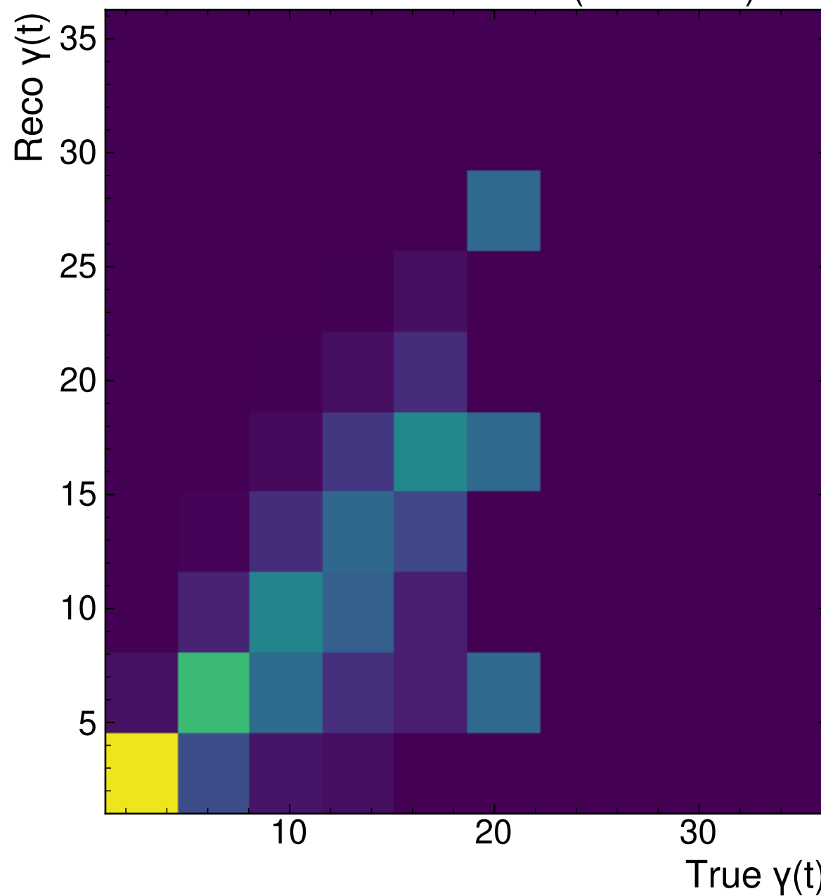
MultiModelTransformer (Magnitude-Direction)
