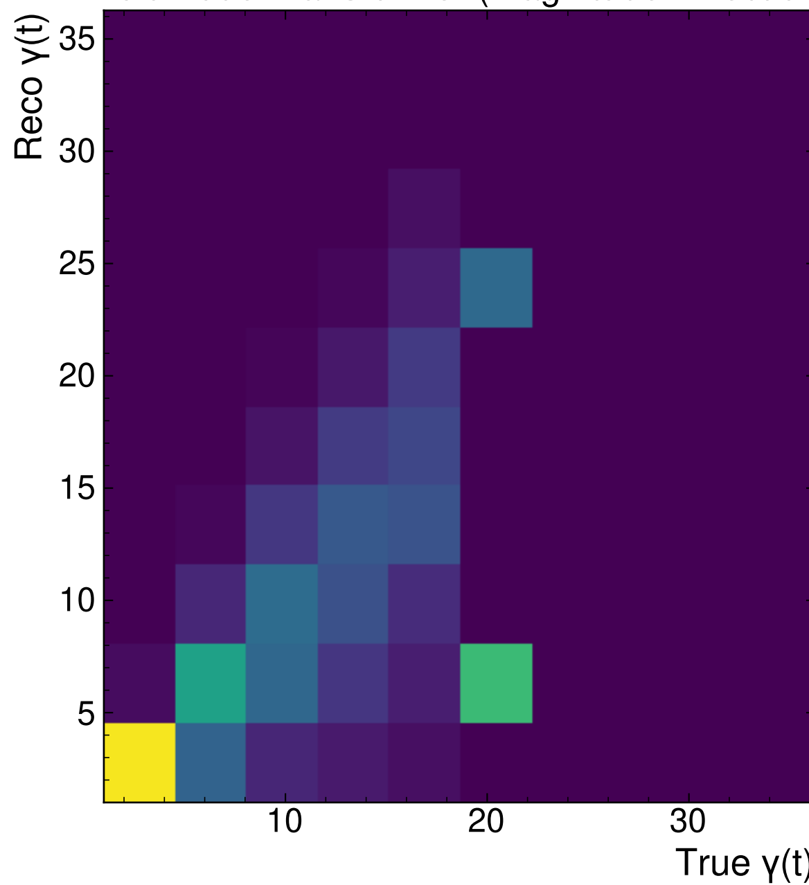
MultiModelTransformer (Magnitude-Direction)
