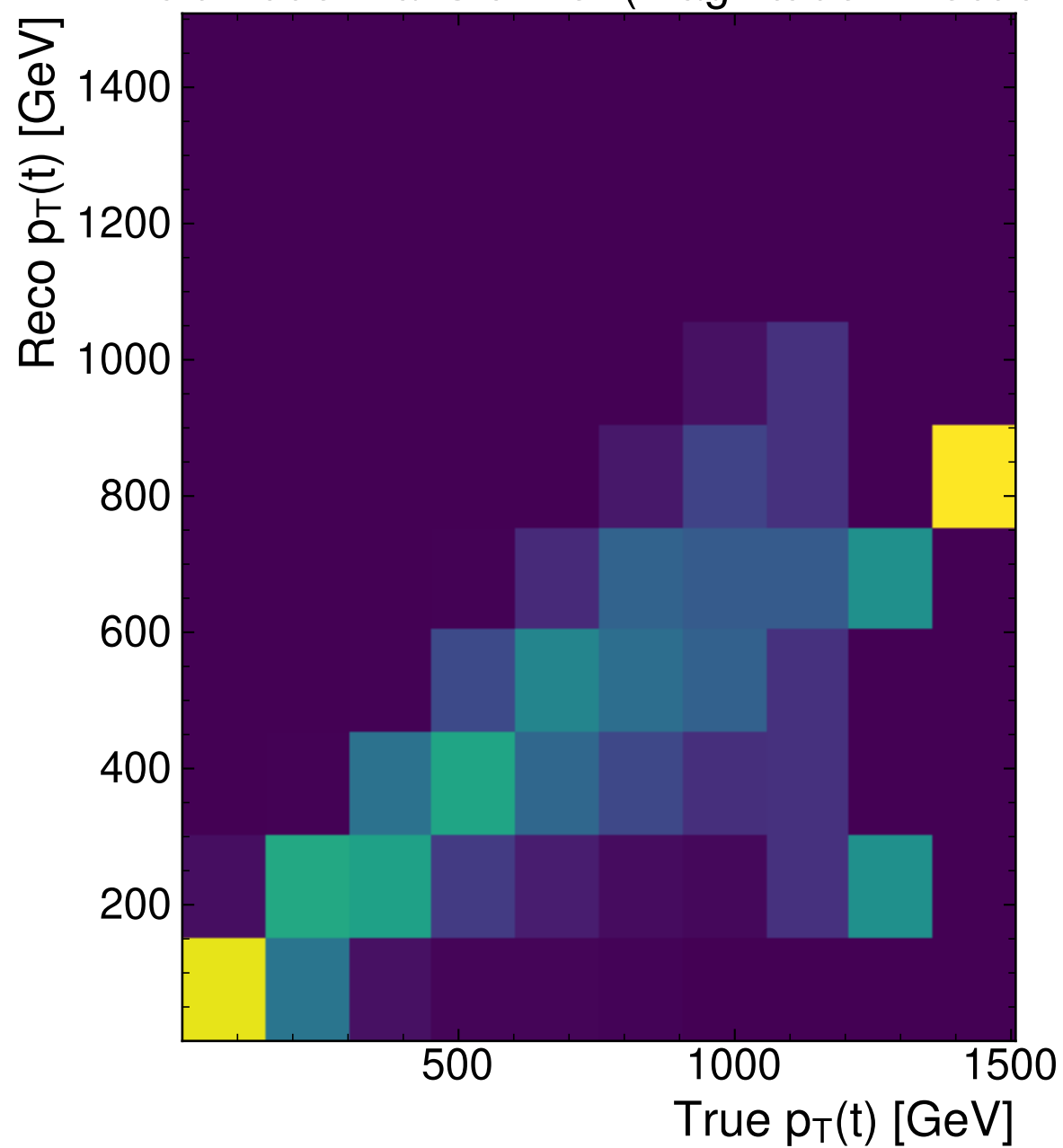
MultiModelTransformer (Magnitude-Direction)
