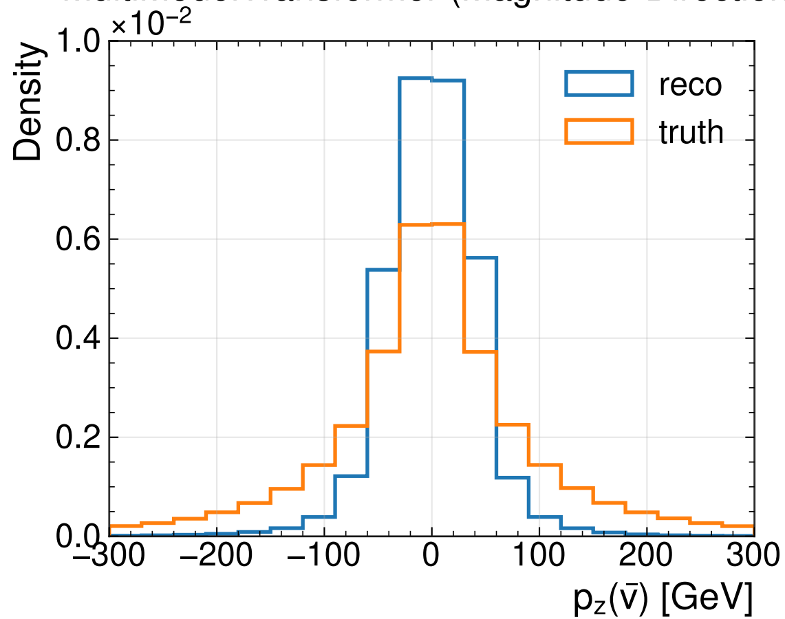
MultiModelTransformer (Magnitude-Direction)
