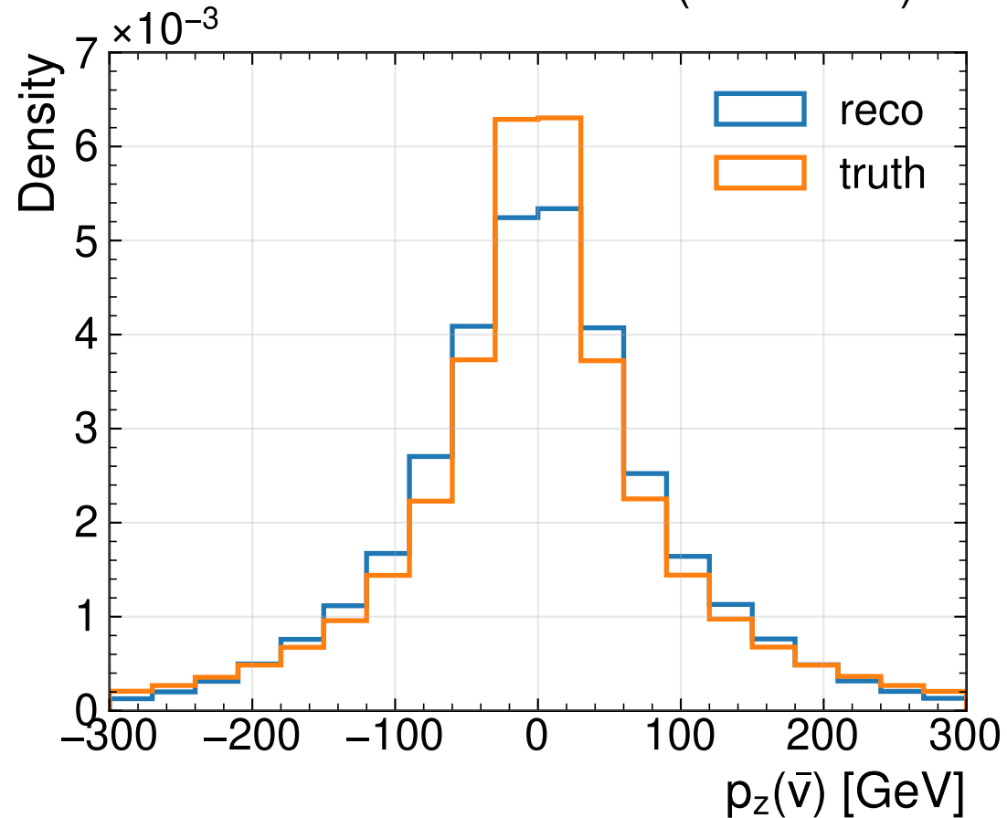
MultiModelTransformer (Magnitude-Direction)
