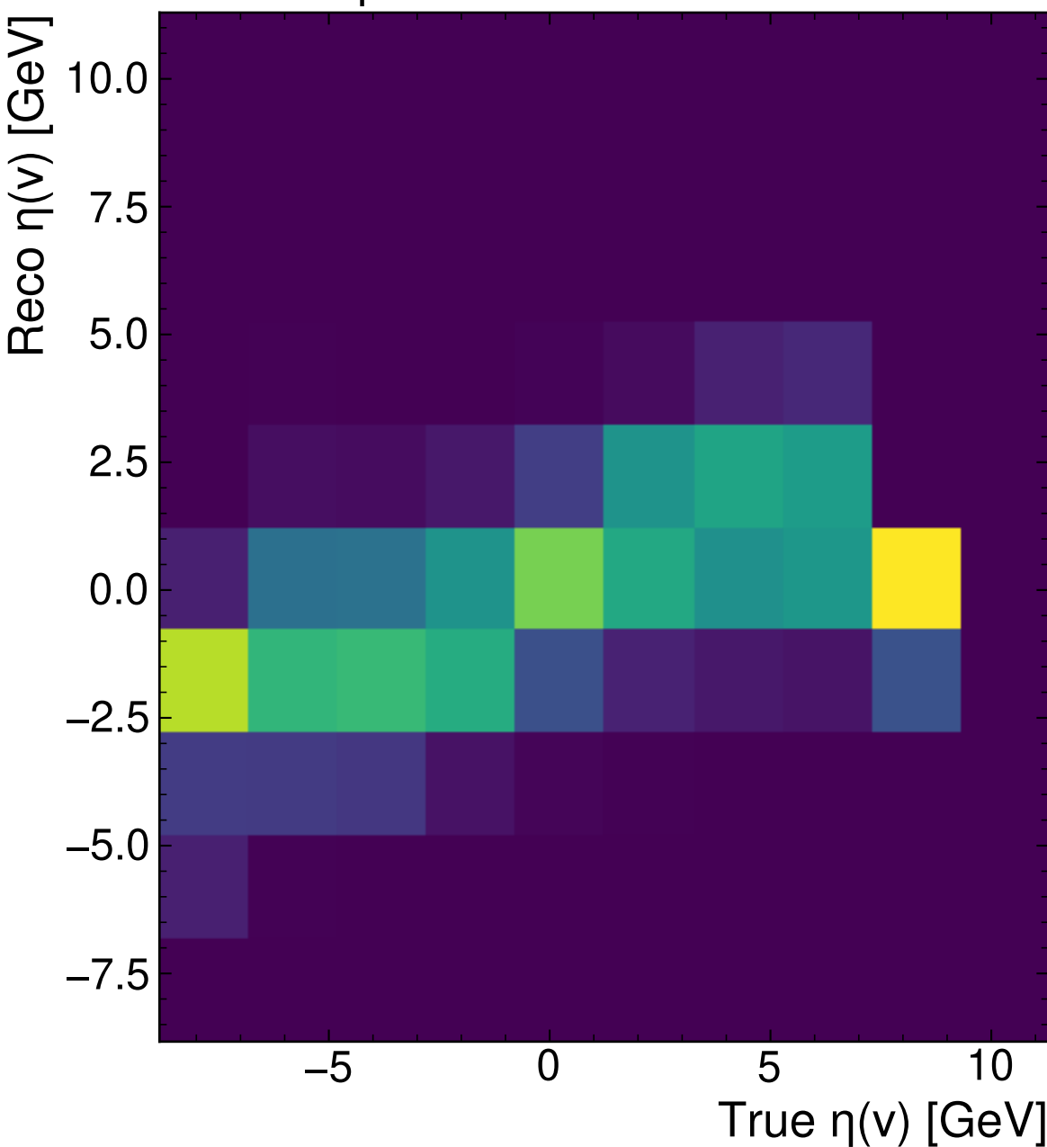
CrossAttentionTransformer + v^2 -Flows
