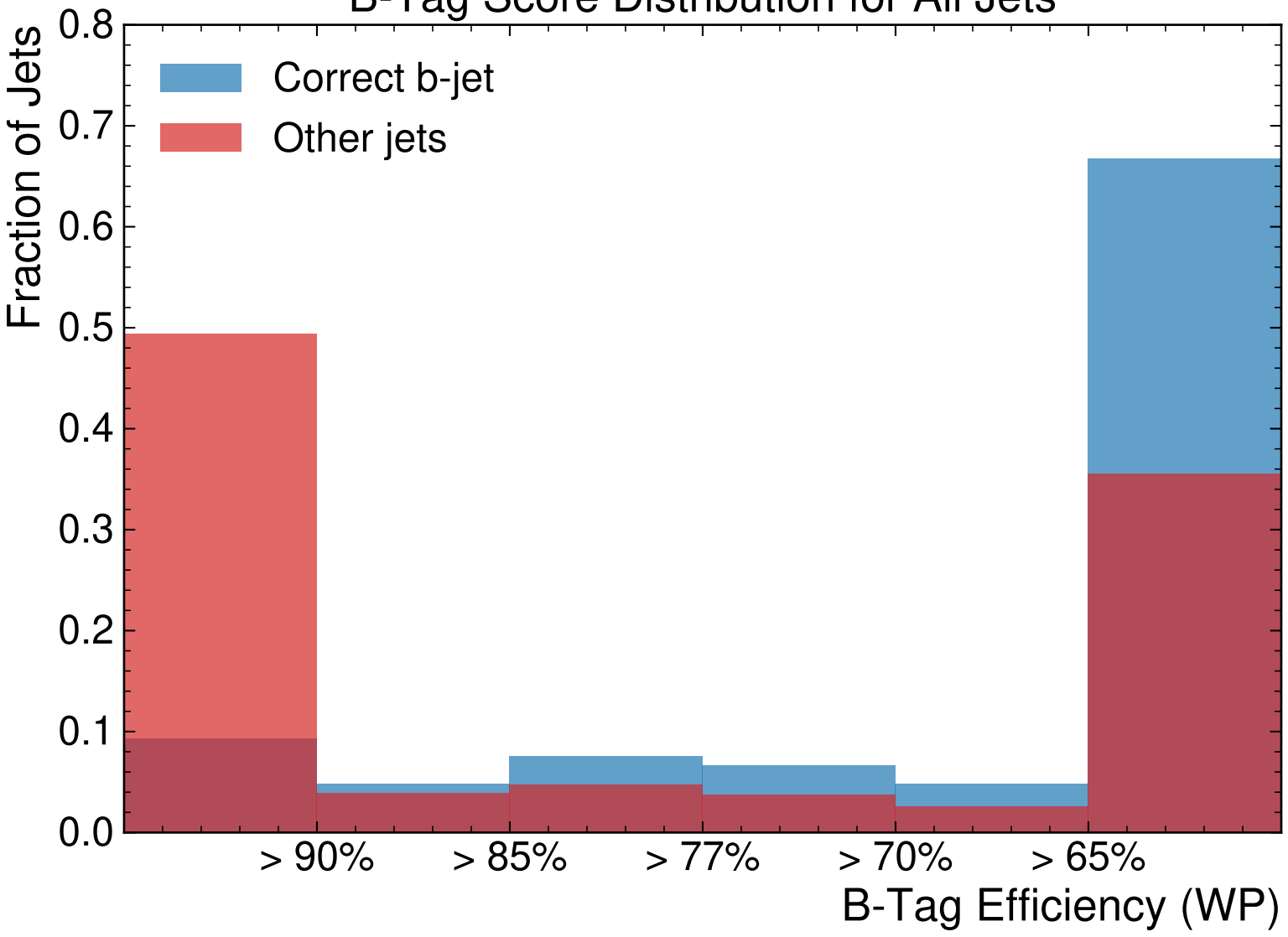
B-Tag Score Distribution for All Jets
