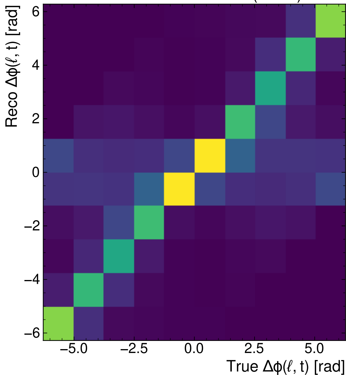
MultiModelTransformer (Mean)
