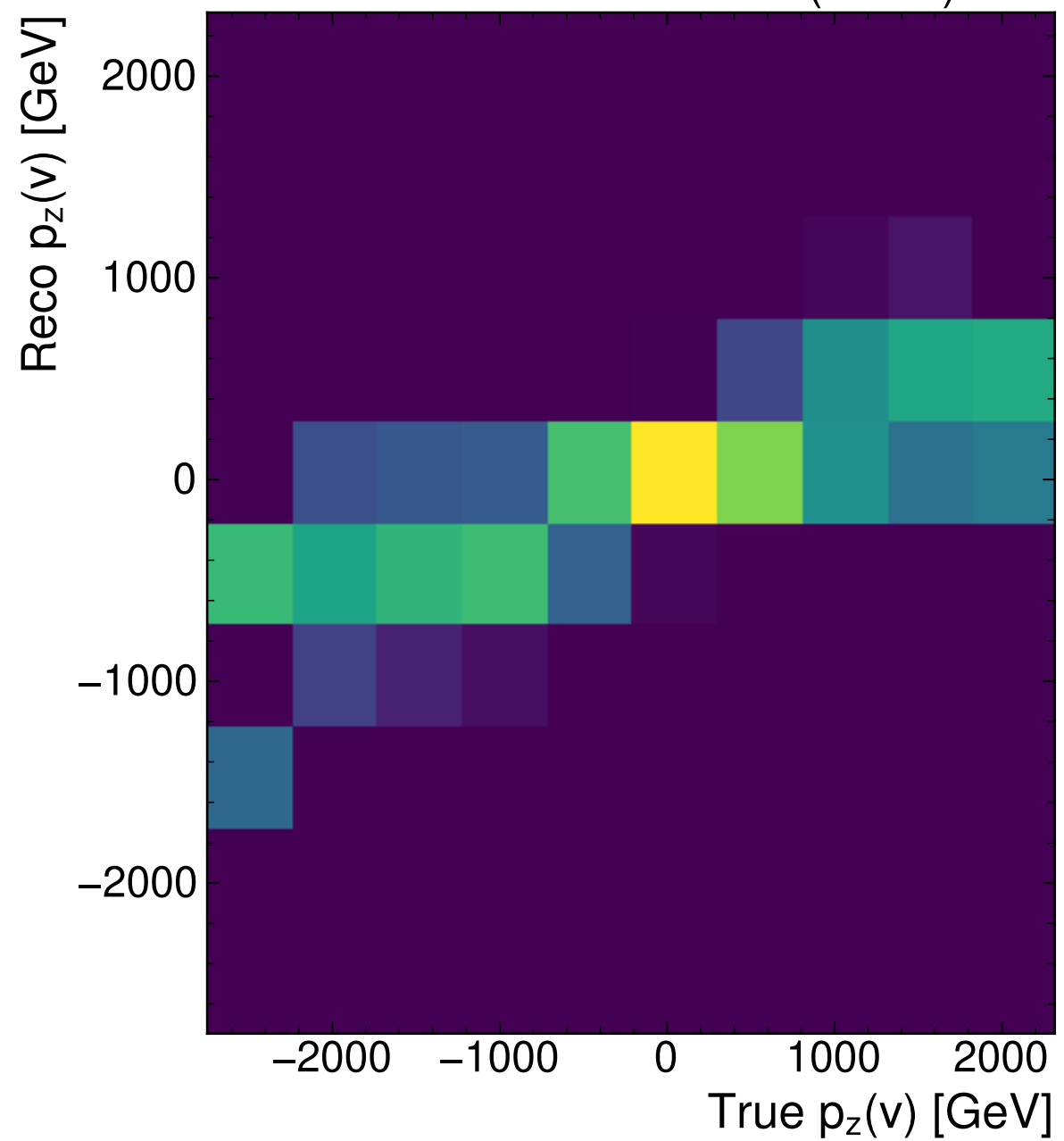
MultiModelTransformer (Mean)
