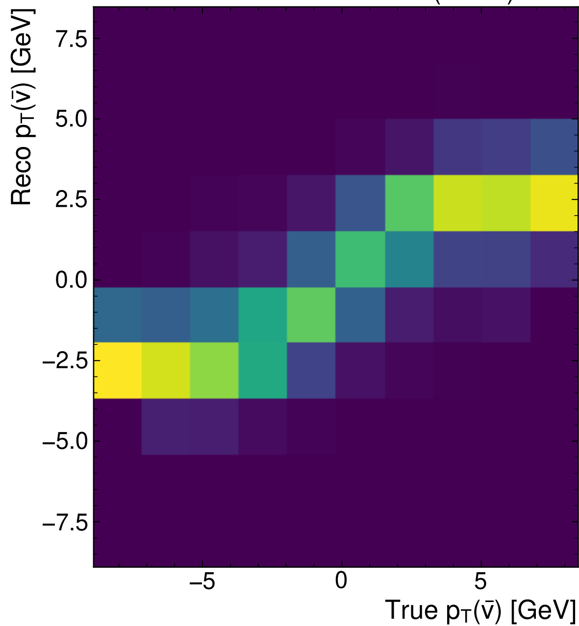
MultiModelTransformer (Mean)
