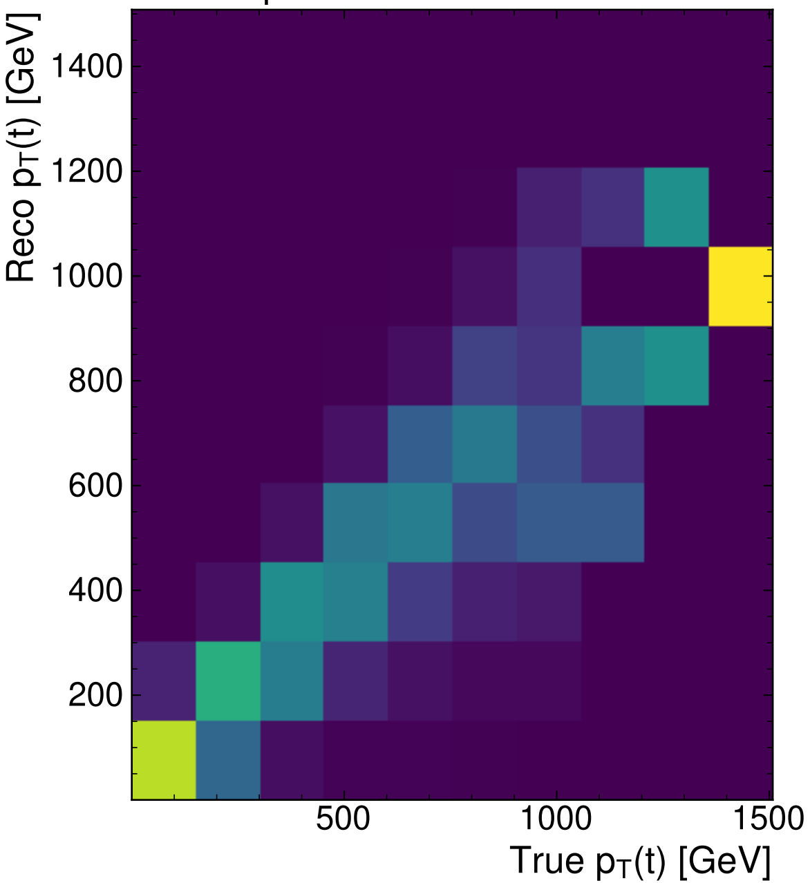
MultiModelTransformer (Gaussian Loss)
