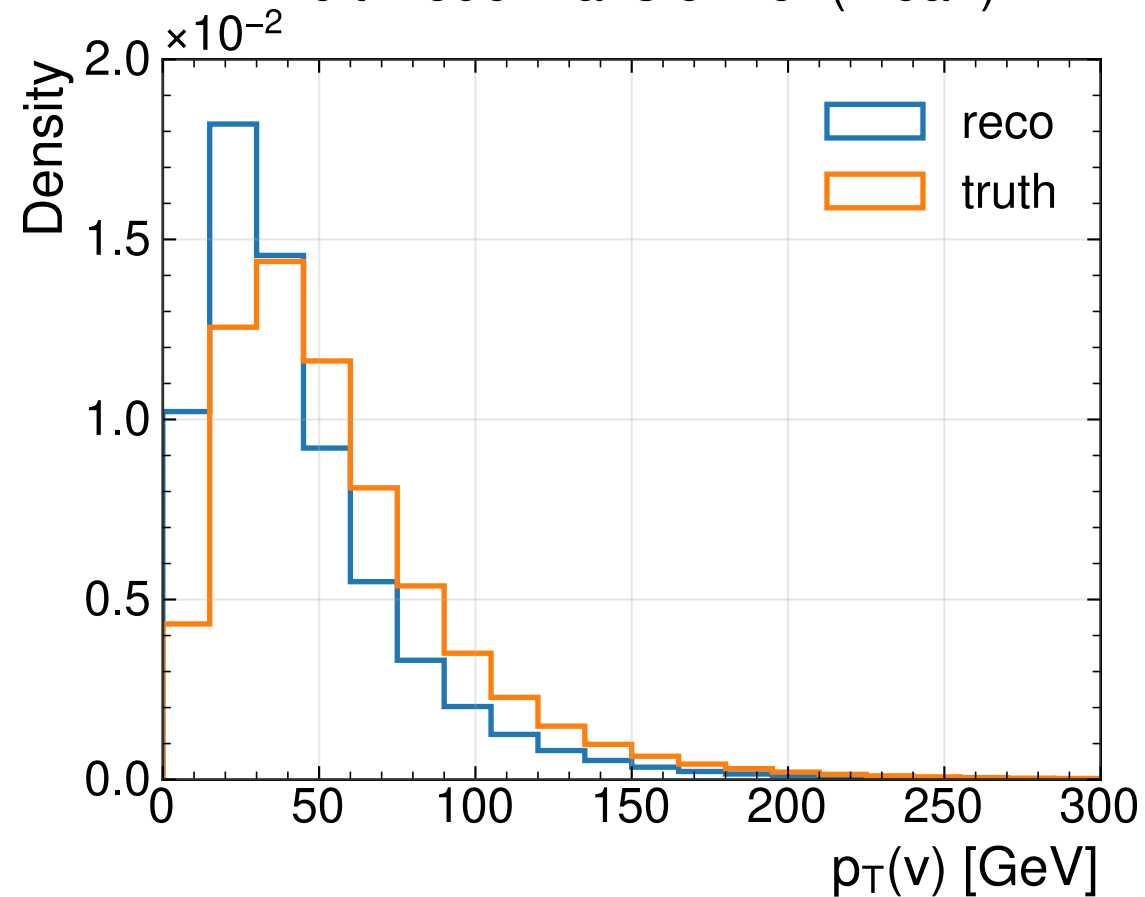
MultiModelTransformer (Mean)
