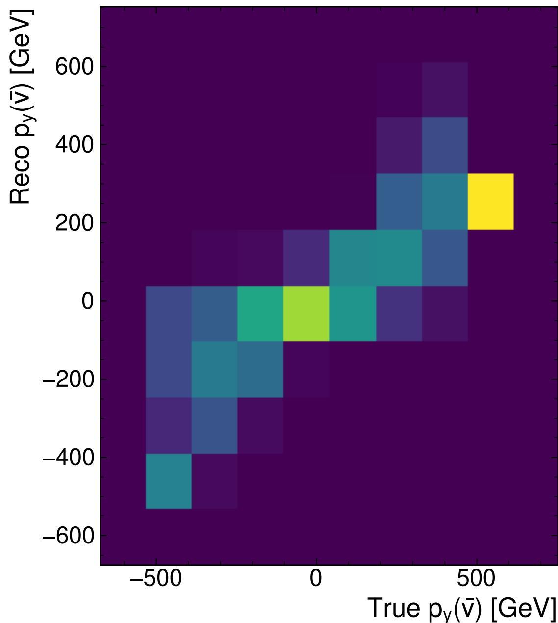
Toponium + v^2 -Flows
