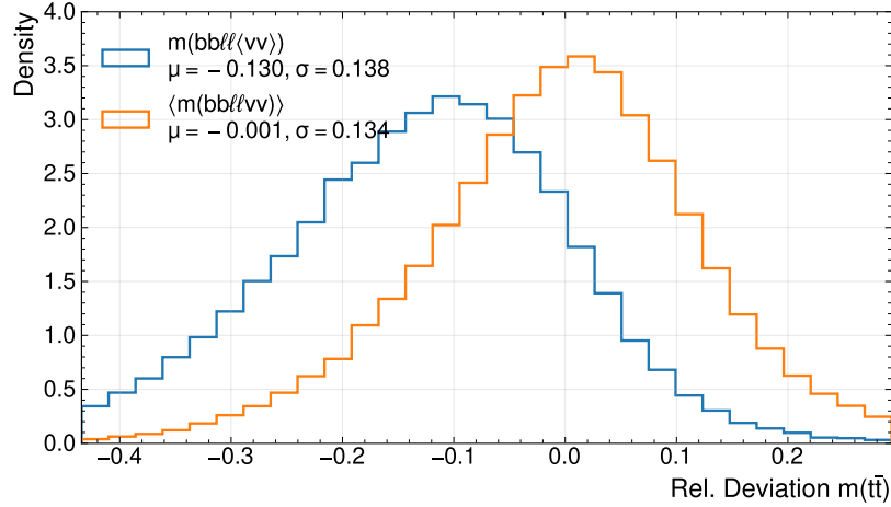
Figure B.2.: Relative deviation between the reconstructed and true m(tt) . The different curves show, whether the invariant mass was computed using the mean momentum or by propagating the neutrino probabilities and averaging of the obtained masses.
