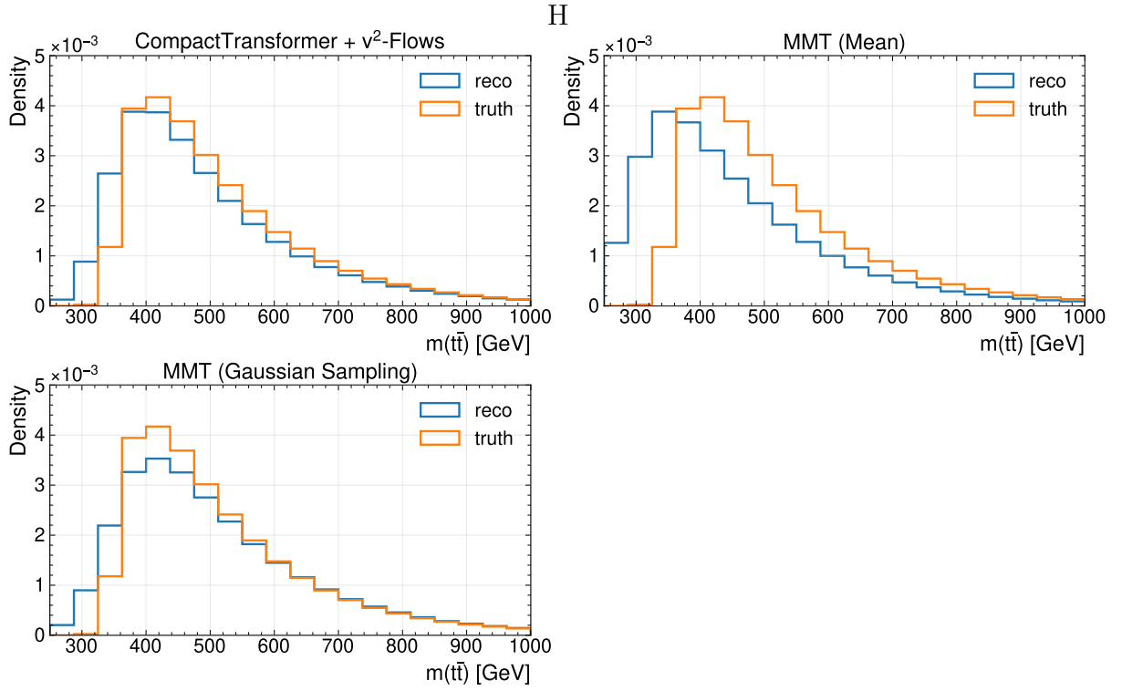
Figure A.21.: Comparison of variable distributions at reco- and truth-level for the different regression settings of the MultiModalTransformer trained with the Gaussian-loss.
