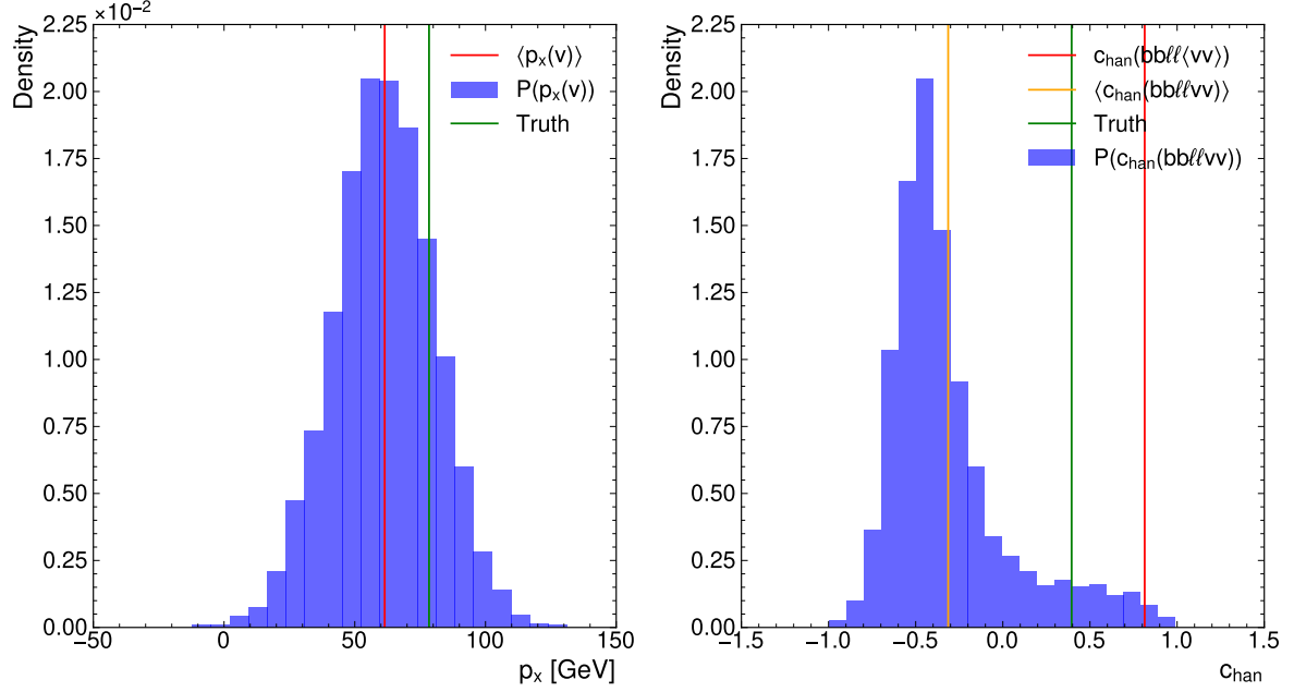
Figure B.5.: Plots showing the probability distribution of the neutrino momentum component p_x and the reconstructed c_{\text{chan}} based on the mean and standard deviation predicted by the MMT-model trained with a Gaussian-loss for a random event. Indicated are the mean and true values.
