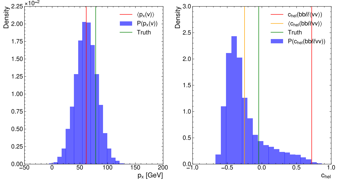
Figure B.3.: Plots showing the probability distribution of the neutrino momentum component p_x and the reconstructed c_{hel} based on the mean and standard deviation predicted by the MMT-model trained with a Gaussian-loss for a random event. Indicated are the mean and true values.
