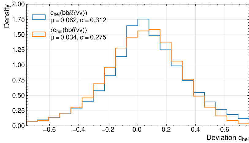
Figure B.4.: Deviation between the reconstructed and true c_{hel} . The different curves show, whether the invariant mass was computed using the mean momentum or by propagating the neutrino probabilities and averaging of the obtained spin-variable.
