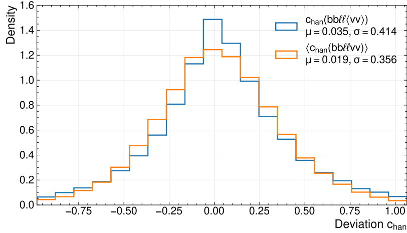
Figure B.6.: Deviation between the reconstructed and true c_{\text{chan}} . The different curves show, whether the invariant mass was computed using the mean momentum or by propagating the neutrino probabilities and averaging of the obtained spin-variable.
