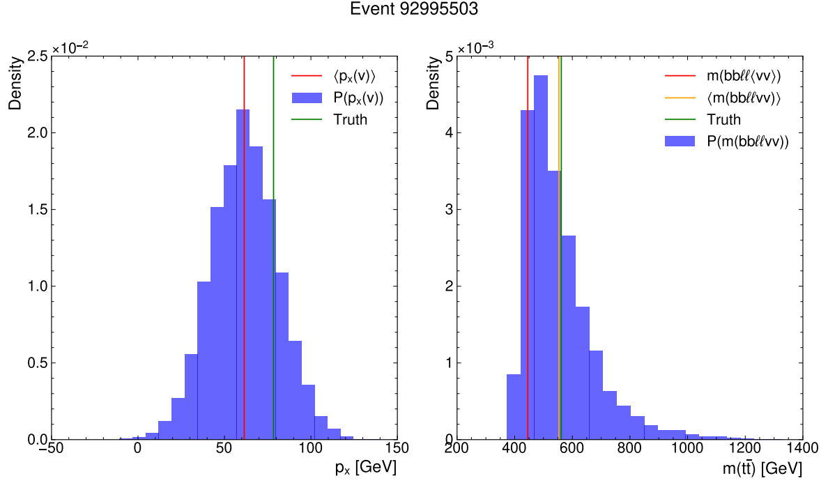
Figure B.1.: Plots showing the probability distribution of the neutrino momentum component p_x and the reconstructed invariant mass m(tt) based on the mean and standard deviation predicted by the MMT-model trained with a Gaussian-loss for a random event. Indicated are the mean and true values.
