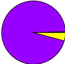
nu_weighter_sr1
