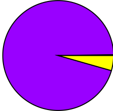
nu_weighter_sr8
