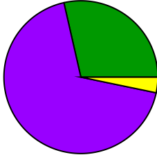
nu_weighter_crZ
