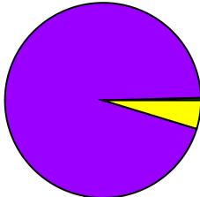
nu_weighter_sr3
