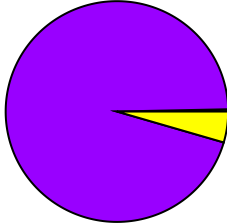
nu_weighter_sr6
