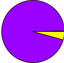
nu_weighter_sr5
