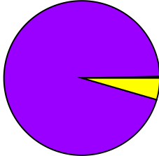
nu_weighter_sr7
