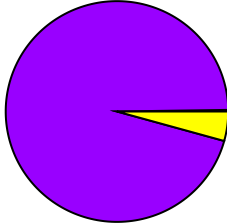
nu_weighter_sr9
