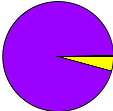
nu_weighter_sr4
