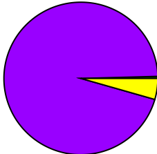
nu_weighter_sr2
