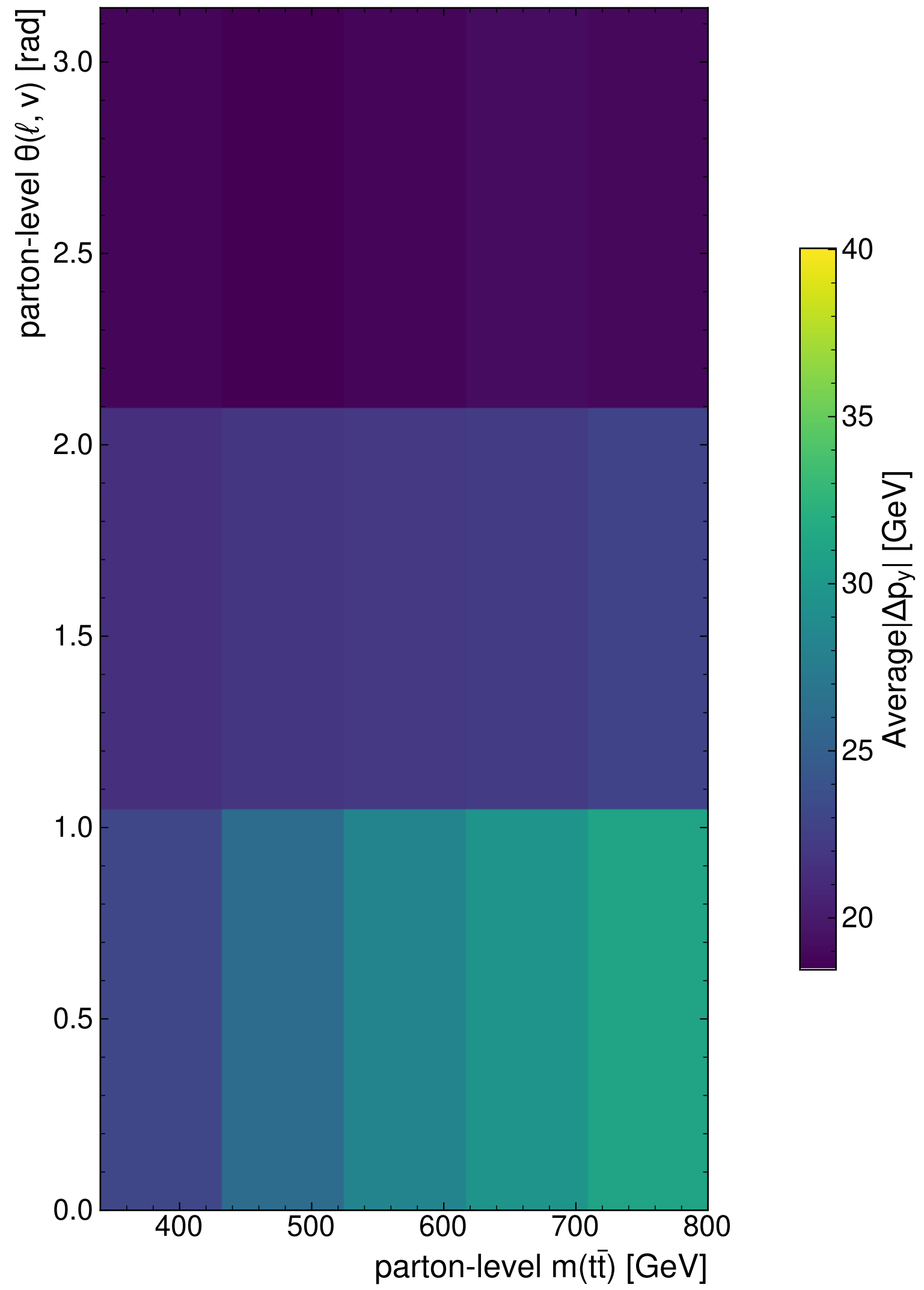
MultiModalTransformer
