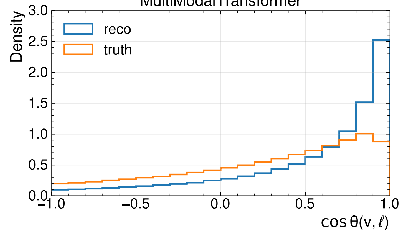
MultiModalTransformer
