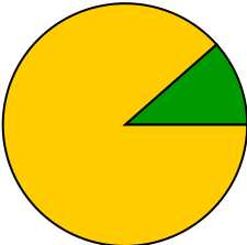
nu_flows_sr_ee
