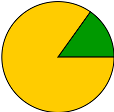
nu_flows_sr_ee
