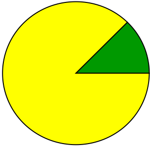
nu_weighter_sr_ee
