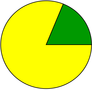
nu_weighter_sr_mumu
