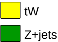
nu_weighter_sr_ee
