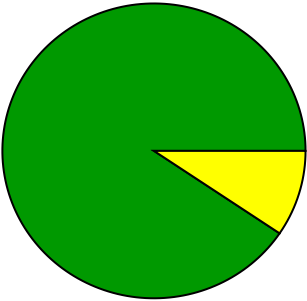
nu_weighter_crZ
