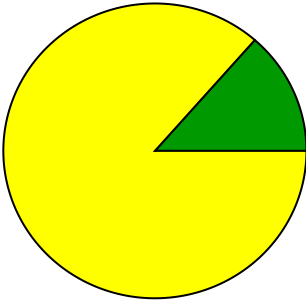
nu_weighter_sr_ee
