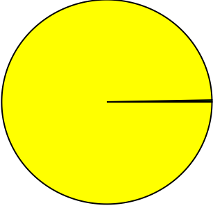
nu_weighter_sr_emu
