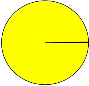
nu_weighter_sr_emu
