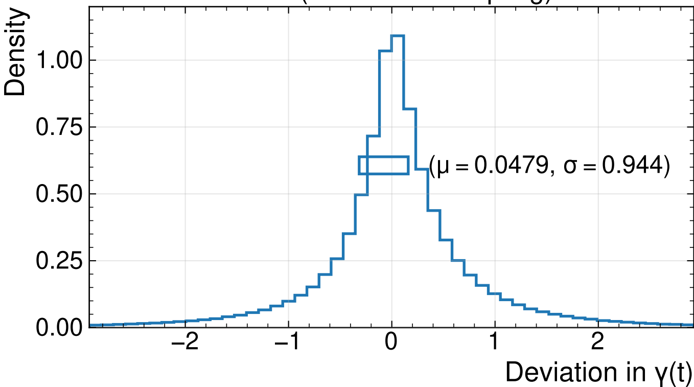
MMT (Gaussian Sampling)
