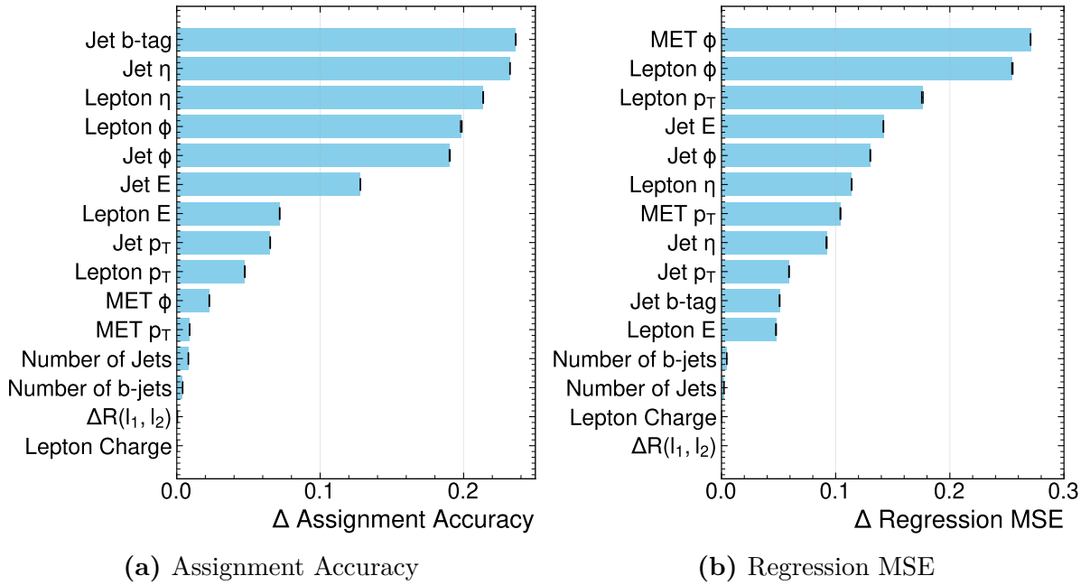
Figure 6.9.: The Plots (a) and (b) show the difference in assignment accuracy and regression MSE, respectively, of the MMT-model when permuting the input features. For each feature, five different permutation are performed. The features are ranked in decreasing order of the observed reduction. Note, that the mean-square error is again computed as the relative deviation of the L^2 -norm as before.
