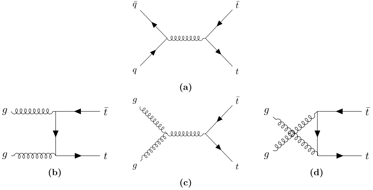
Figure 2.3.: Leading order Feynman diagrams for top-quark pair production in (a) quark-antiquark annihilation and (b), (c) & (d) gluon fusion (ggF).
