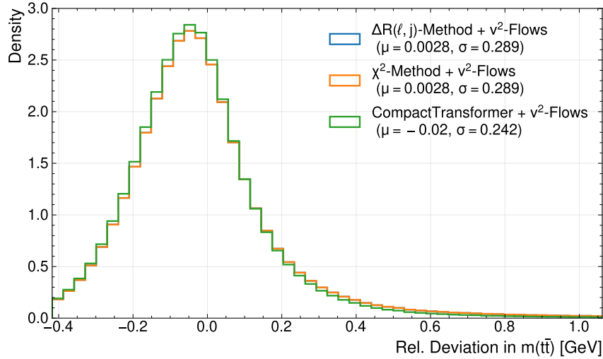
Figure 7.10.: Plot showing the relative deviation of the invariant mass reconstruction. The legend includes the obtained mean and standard deviation, which correspond to the resolution, for each method.
