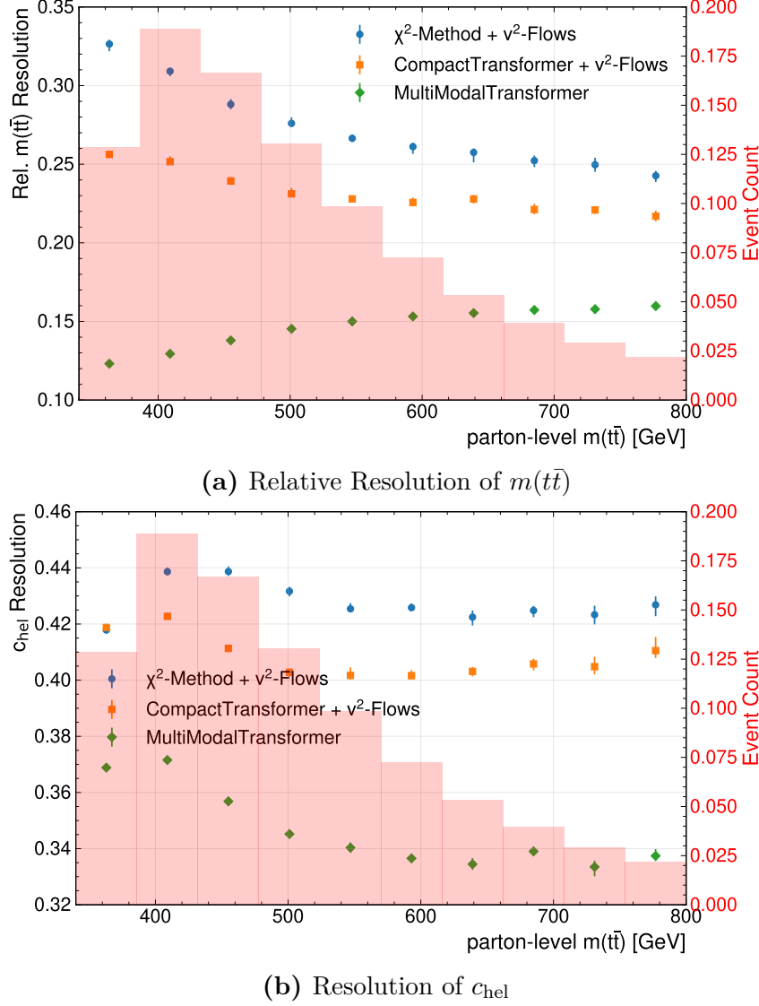
Figure 7.14.: (Relative) Resolution of m(t\bar{t}) (a) and c_{\text{hel}} (b) computed in bins of the parton-level invariant mass of the t\bar{t} -system. Different setups for assignment and regression are compared.
