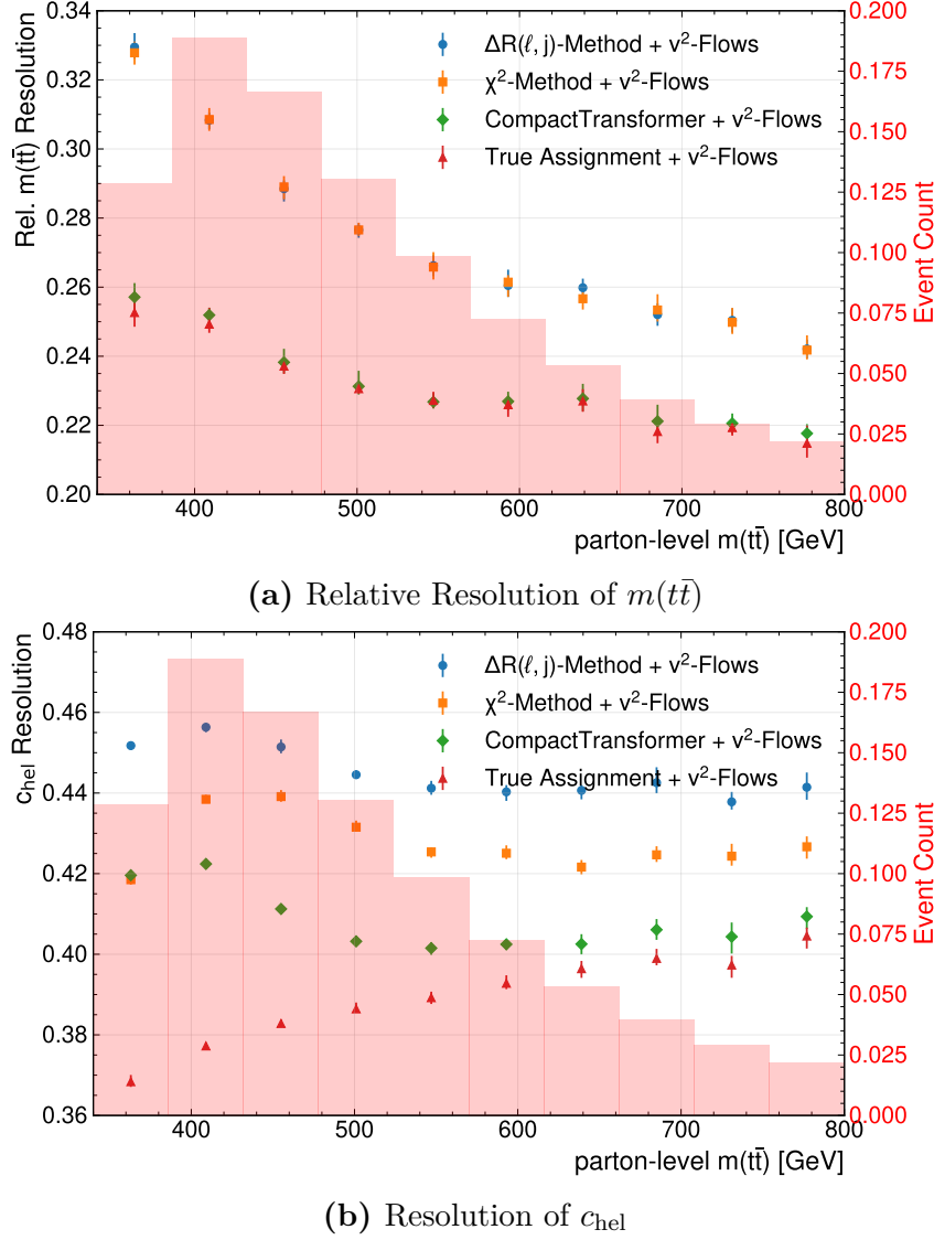
Figure 7.11.: (Relative) Resolution of m(t\bar{t}) (a) and c_{\text{hel}} (b) computed in bins of the parton-level invariant mass of the t\bar{t} -system. The different methods, as well as the expected resolution with perfect efficiency for the assignment, are compared. The displayed error bars represent the statistical uncertainties of the dataset obtained via bootstrapping.
