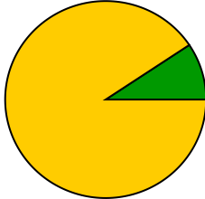
nu_weighter_cr_ll
