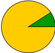
nu_weighter_cr_ll
