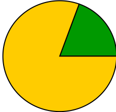
nu_weighter_cr_mumu
