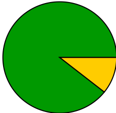
nu_weighter_crZ
