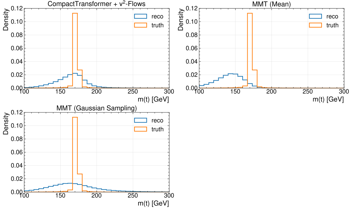
Figure A.24.: Comparison of m(t) distributions at reco- and parton-level for the different regression settings of the MultiModalTransformer trained with the Gaussian-loss.
