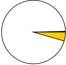
nu_flows_sr8
