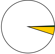
nu_flows_sr6
