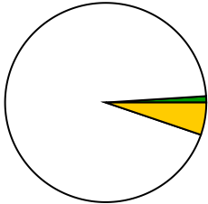
nu_flows_sr3
