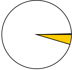
nu_flows_sr9
