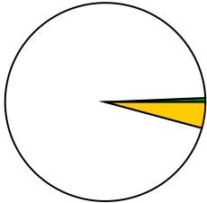
nu_flows_sr1
