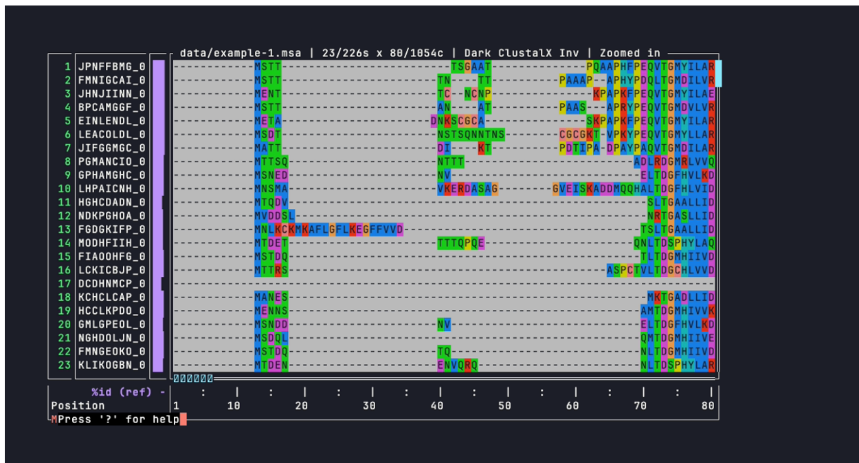
Figure 1: Termal displaying example-1.msa. From left to right and top to bottom: headers pane, alignment pane, corner pane, reference pane, and modeline.
