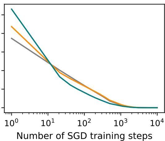
\ell^2 -distance to limit point
