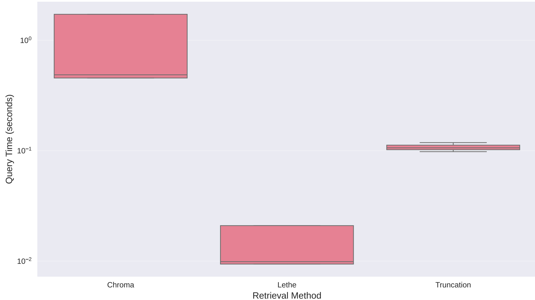
Query Time Comparison - InfinityBench zh.qa
