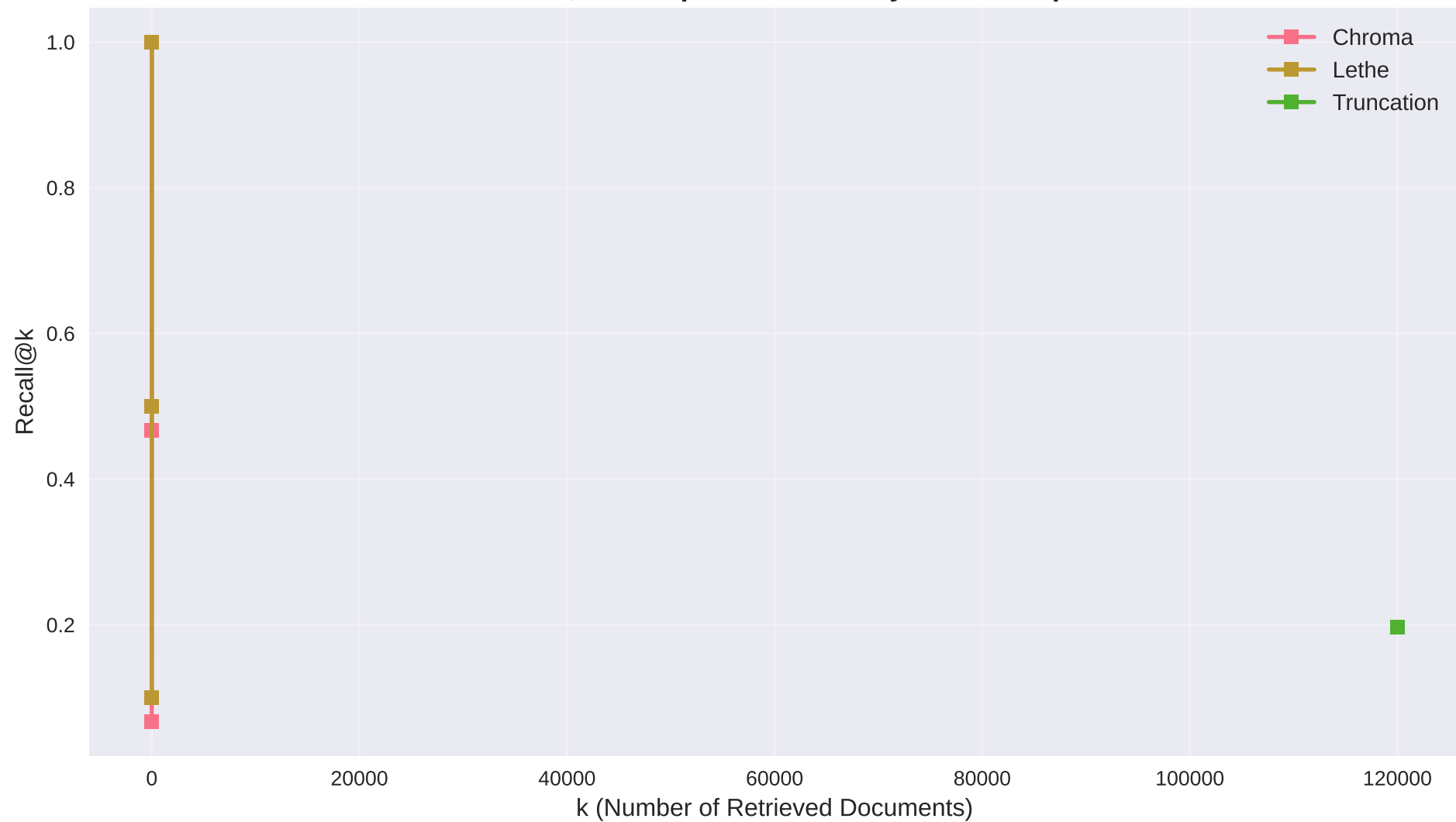
Recall@K Comparison - InfinityBench zh.qa
