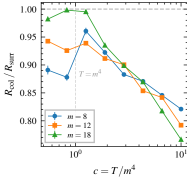
(b) Regret ratio
