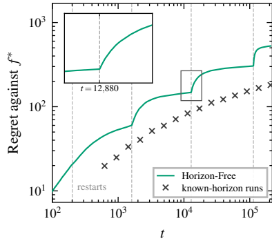
(c) Horizon-free, m = 12
