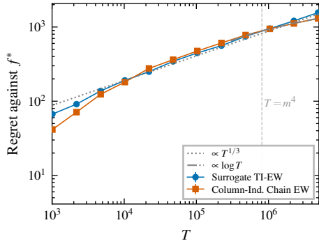
(a) m = 30
