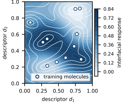
kriging posterior over two descriptors (filled = mean, white = sd)
