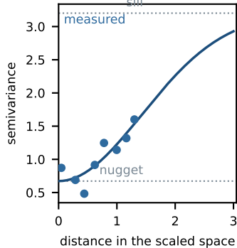
\gamma(h) from the plant campaign, nugget/sill = 0.21
