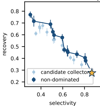
inversion: candidates ranked on the trade-off, with uncertainty
