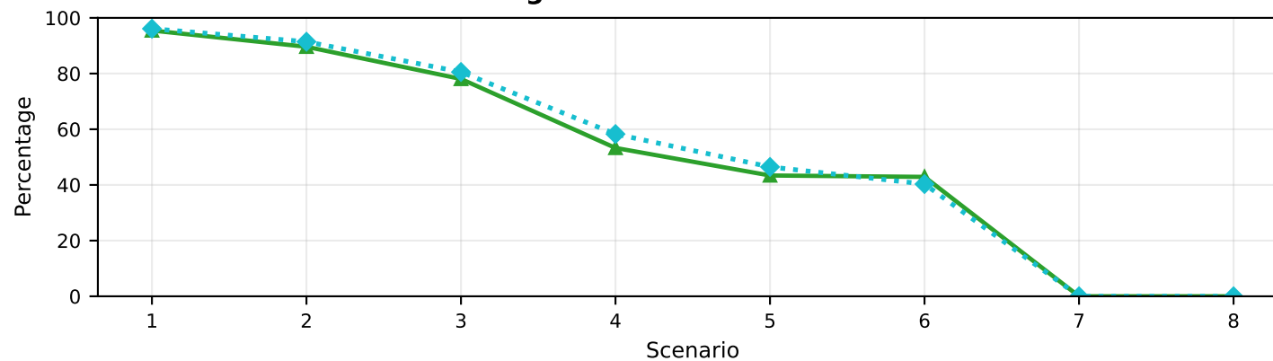
E. Percentage of administrations underdosed
