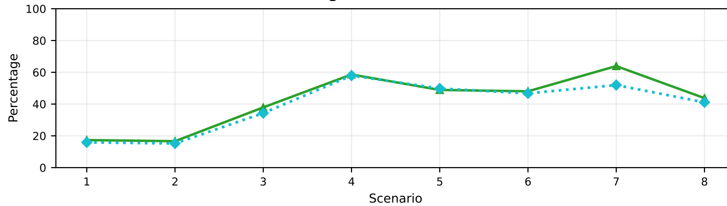
A. Percentage of correct MTD selection
