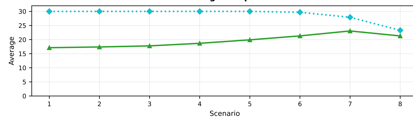
G. Average sample size
