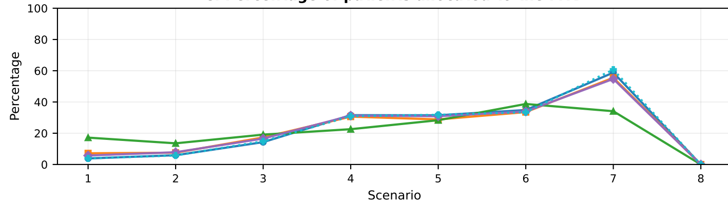
C. Percentage of patients allocated to the MTD
