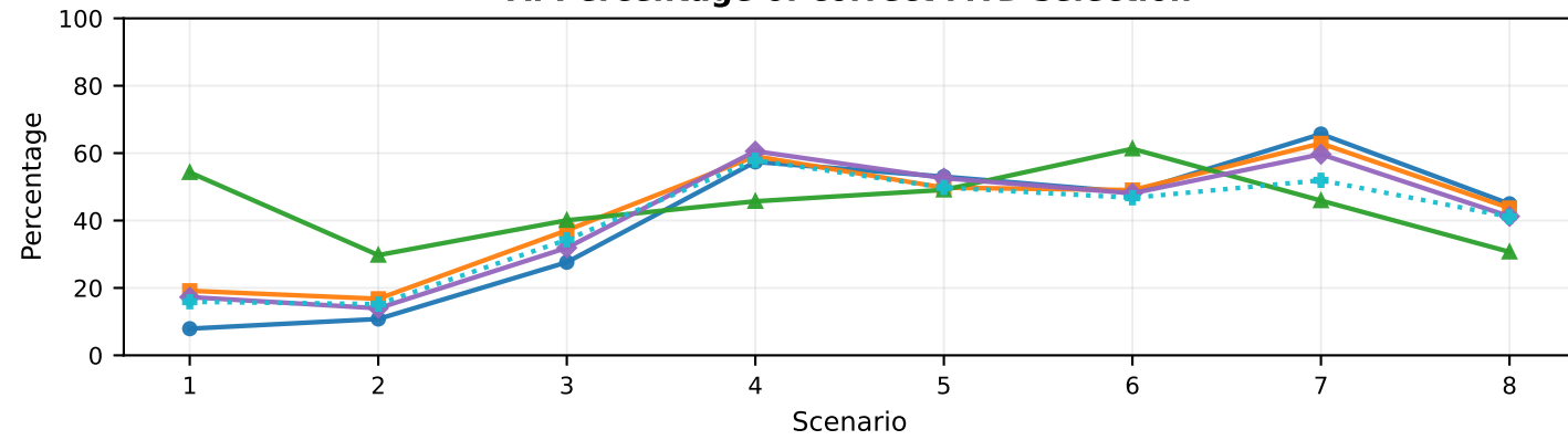
A. Percentage of correct MTD selection
