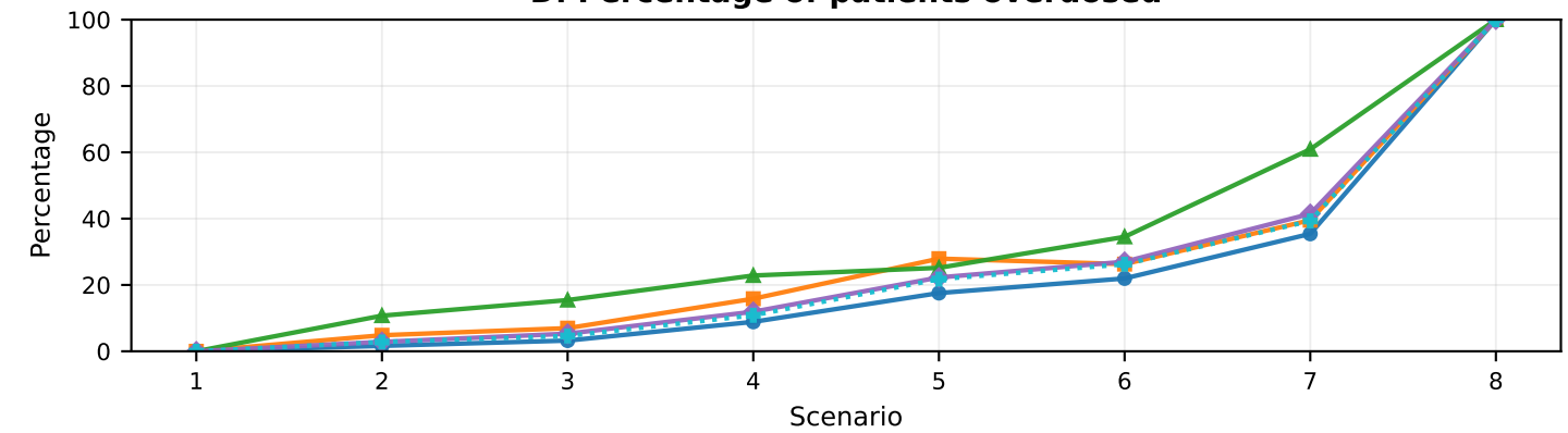
D. Percentage of patients overdosed
