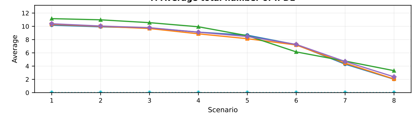
F. Average total number of IPDE
