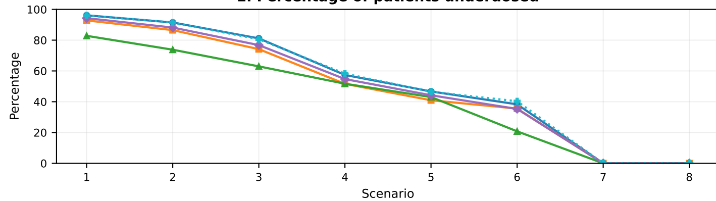
E. Percentage of patients underdosed
