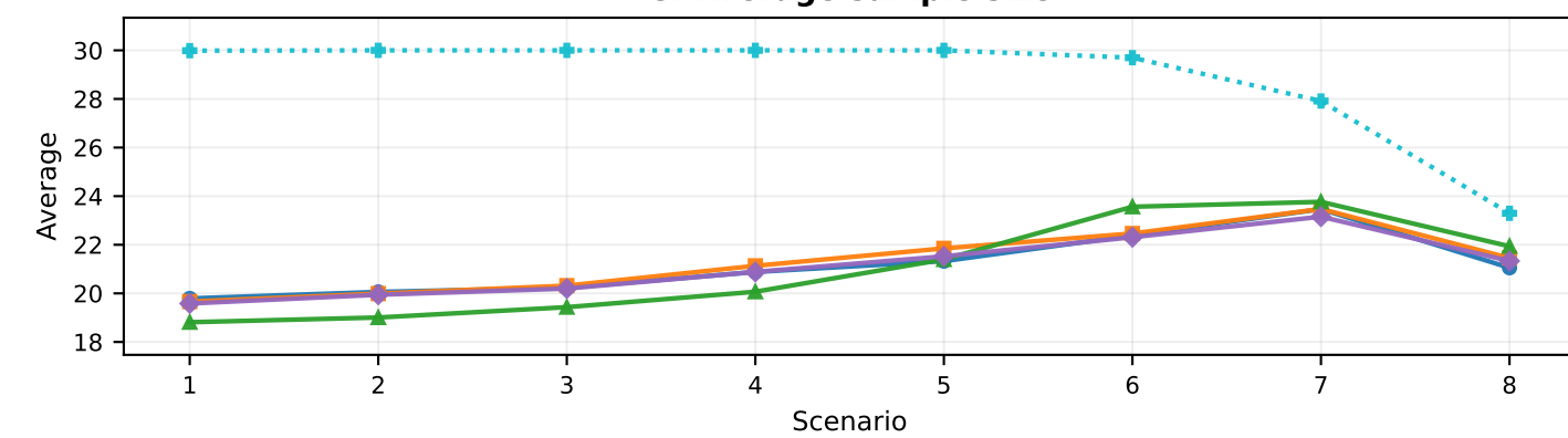
G. Average sample size
