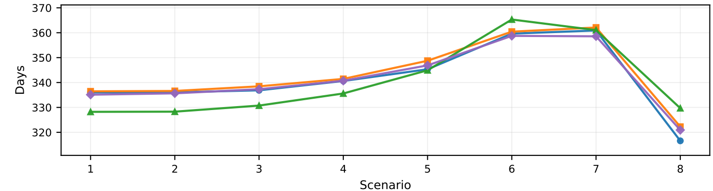
H. Average trial duration
