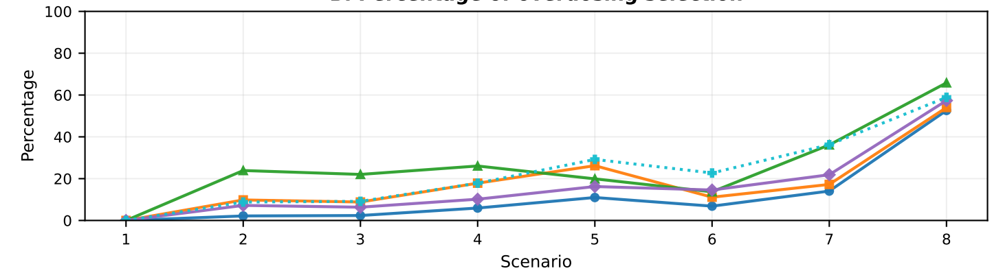
B. Percentage of overdosing selection
