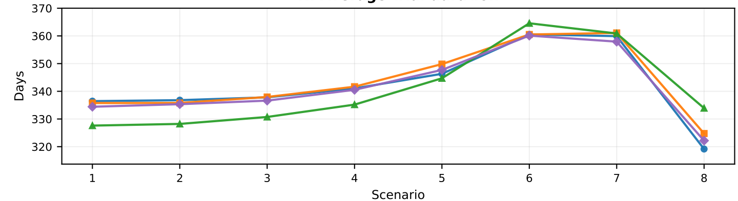
H. Average trial duration
