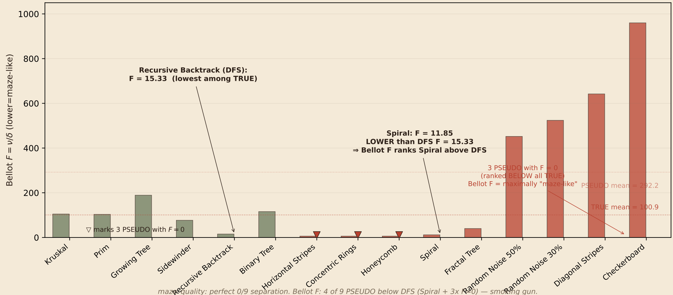
(b) Bellot F (Bellot 2021 §3.4): TRUE mean = 100.9, PSEUDO mean = 292.2, gap = -191.3. 4 of 9 PSEUDO score LOWER than DFS — direct failure.
