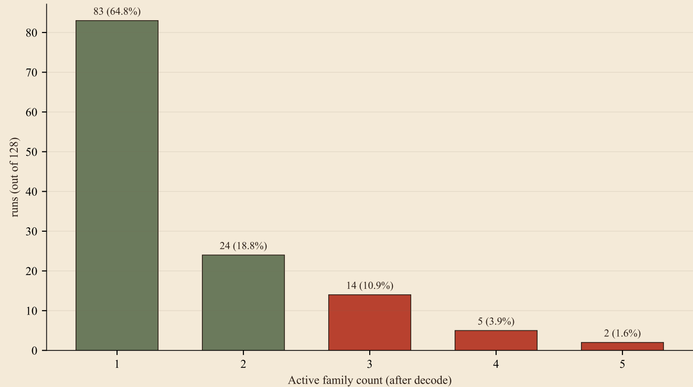
Active family distribution in 128-run sweep (64.8% collapse to 1 family; ES prefers “less is more”)
