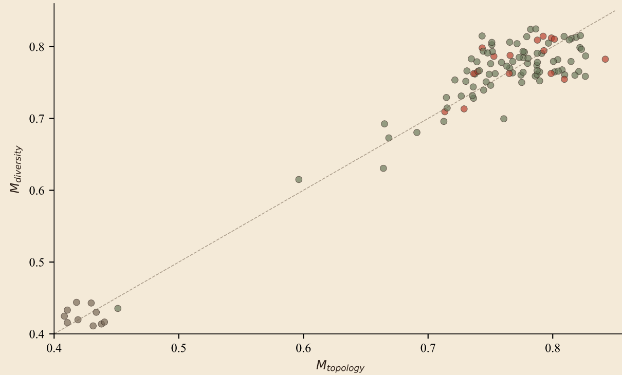
(C) Topology vs diversity (dashed: y = x )
