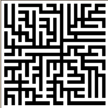
Growing Tree
