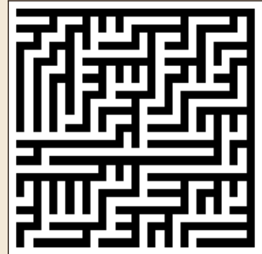
Binary Tree
