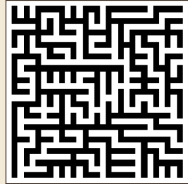
Binary Tree
