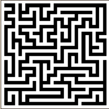
Growing Tree
